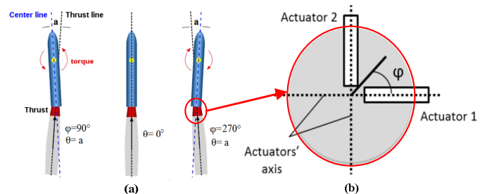
Fig.1 : Considered Thrust Vector Control system (TVC). (a) Torque generation for 3 inclination cases of the thrust, (b) Upper view of actuators axis and inclination angle \varphi .
