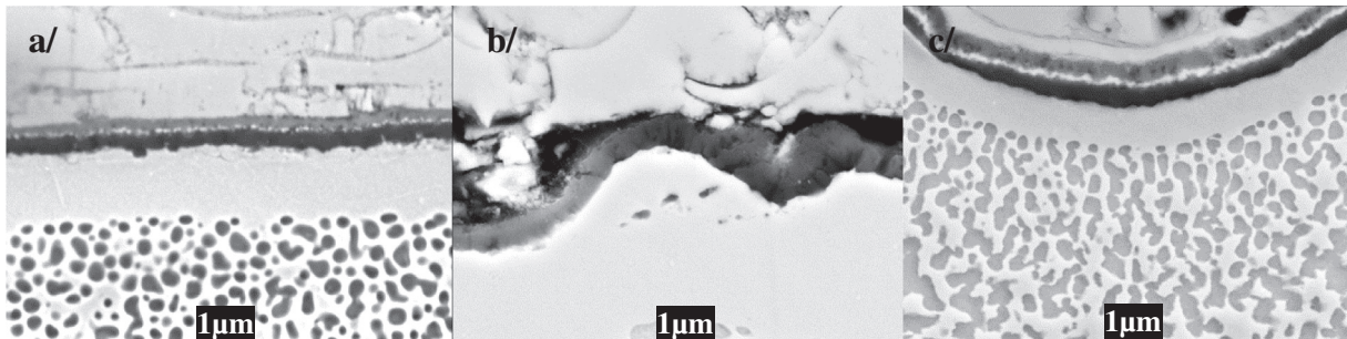
Fig. 4. Cross-sections for polished (a), grit-blasted (b) and laser treated (c) samples after 100 h of isothermal oxidation at 1100^\circ\text{C} – from top to bottom: TC (light), spinel (grey), alumina oxide (dark) and substrate (light).
