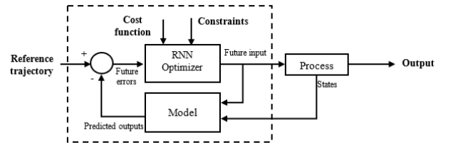
Figure 5: Block diagram of our proposed control scheme
