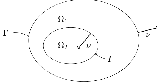
FIGURE 1. The set \Omega = \Omega_1 \cup I \cup \Omega_2 .
