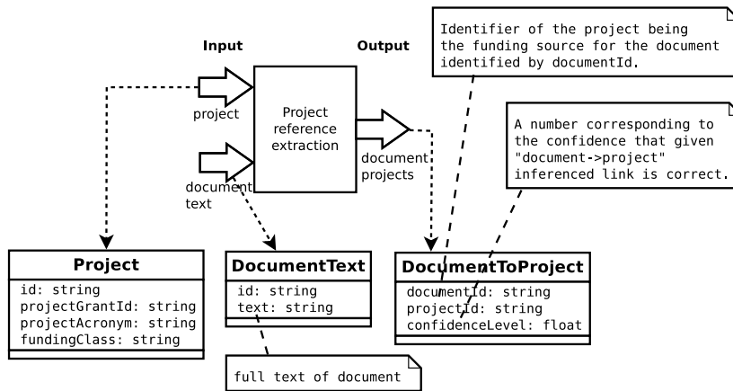
Fig. 1. A sample OpenAIREplus workflow node that ingests data stores corresponding to projects and full text of documents and produces a data store containing links between documents and projects. The node specifies its inputs and outputs with Avro schemas, which are represented here as UML class diagrams.
