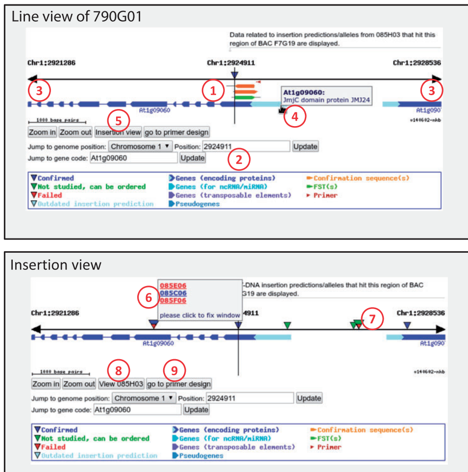
Fig. 1 Summary of features of the updated visualization component. There are several ways to access the visualization component, usually via a click on one of the triangles somewhere in the SimpleSearch content. There are two views to the visualization: the 'Line view' (top) and the 'Insertion view' (bottom). The 'Line view' can be accessed when coming from inspecting the details of a specific line. In this case, only primers, confirmation sequences and insertion predictions (triangles) are displayed that correspond to the line selected (1). The user can navigate in the visualization by entering a position or an AGI locus code (2), or by scrolling through the genome using the arrowheads (3). Further information is provided by tooltips (4), and by links to pages within SimpleSearch (a click on the symbols for primers, FSTs, confirmation sequences or the triangles representing lines causes calling the respective information) or to Araport for genes. Since annotation units/BACs are not supported by Araport11, these are linked to TAIR. To access the 'Insertion view,' the respective button can be used (5). This view shows all insertions within the selected range without FSTs, confirmation sequences and primers that are related to a specific line/insertion allele. When there are multiple insertions close to each other, they are displayed in a larger triangle. These larger triangles might show multiple colors if there are confirmed and failed insertion alleles (originating from a contamination) at nearby positions (6); other color combinations in the larger triangles are also possible (7). When the visualization was initially started in the line view, it is possible to switch back (8). It is also possible to switch to the primer design tool (Huep et al. 2014) to generate primers for the selected position (9).
