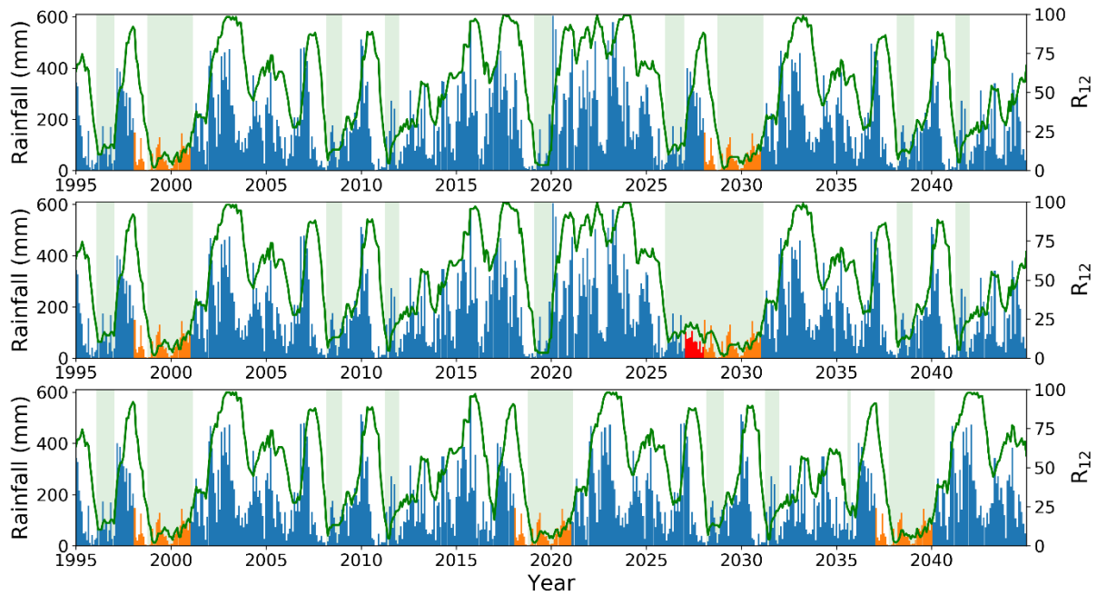
Figure 2. Monthly rainfall for the period January 1995 to December 2044 for rainfall scenarios (a) S1, (b) S2, and (c) S3. The green line shows the R_{12} trends for the rainfall time series, where R_{12} is obtained by first summing the month's rainfall and that of the preceding 11 months, and ranking this relative to other 12-month sums (Post et al., 2018). The green shading indicates periods with R_{12} < 25\% . The orange bars are used to highlight the replicated 1998 – 2000 drought period. The red bars indicate the values used for the year 2027 in rainfall scenario S2, in which each month was the average of the corresponding month in the years 2025, 2026, 2028, 2029 and 2030.
