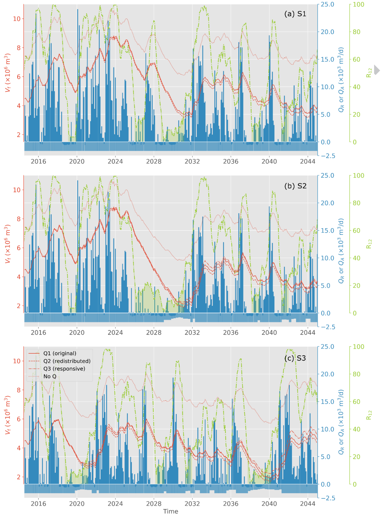
Figure 6. Results of model simulations for rainfall scenarios: (a) S1, (b) S2, (c) S3. The lens volume ( V_f ) is shown in red, whereby solid lines, dotted lines and dashed lines are for, respectively, the abstraction regimes of pumping at the original design yield (Q1), pumping redistribution (Q2), and
