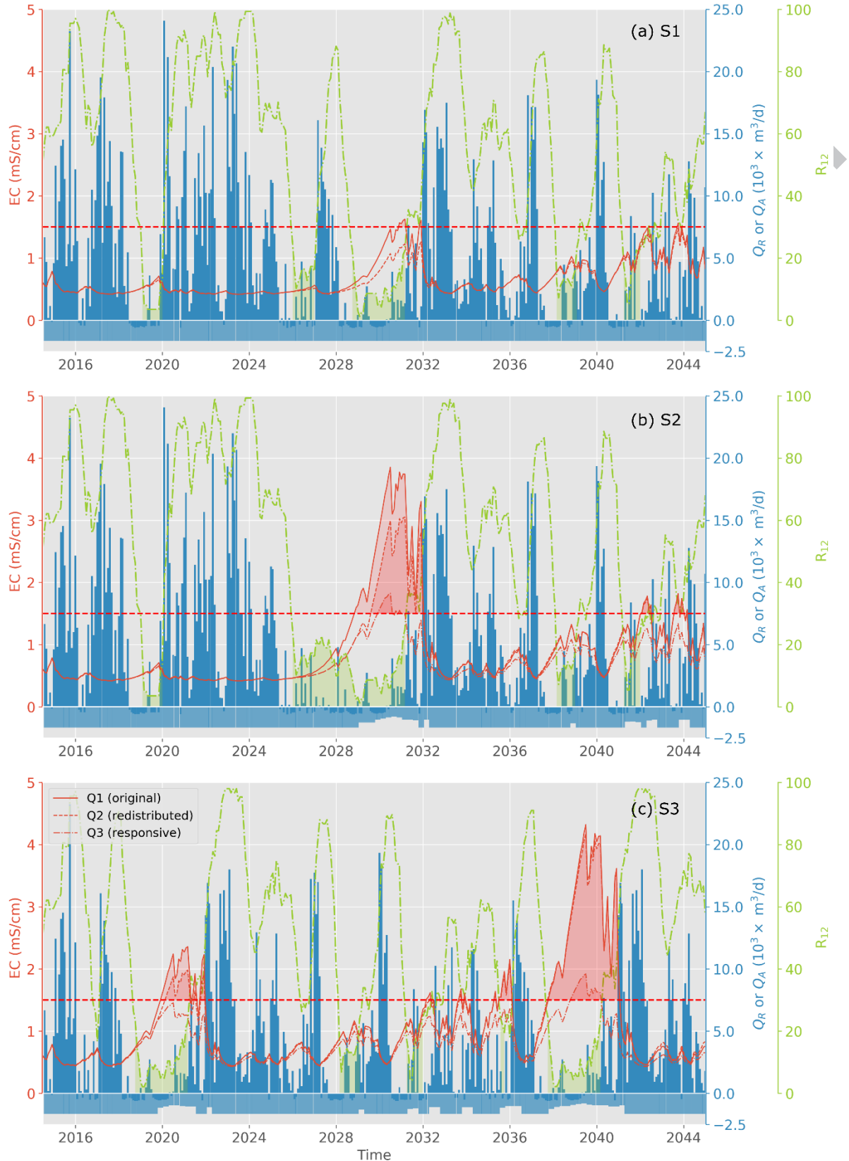
Figure 5. Results of model simulations for rainfall scenarios: (a) S1, (b) S2, and (c) S3. The EC is shown in red, whereby solid lines, dotted lines and dashed lines are for, respectively, the abstraction regimes of pumping at the original design yield (Q1), pumping redistribution (Q2), and pumping
