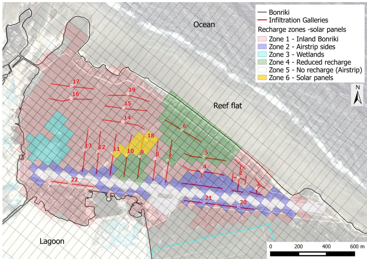
Figure 3. Zonation of recharge in the numerical simulations and the location of infiltration galleries, overlain on a close-up of the model grid. The yellow area indicates zone 6, which experienced higher recharge rates since September 2015 when the vegetation was cleared and solar panels were installed. Prior to this, it was part of recharge zone 1.
