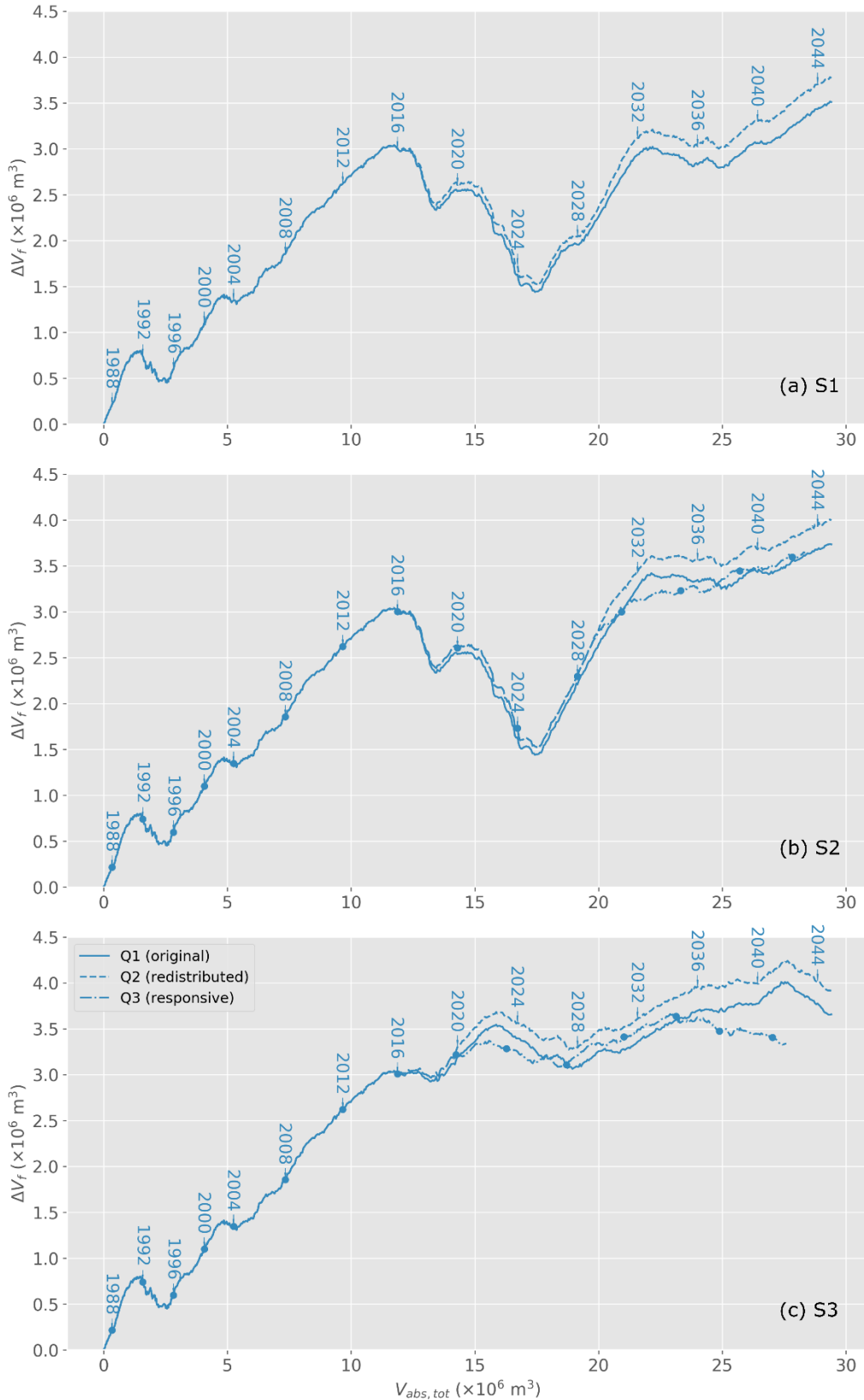
Figure 7. Graph showing the pumping-induced depletion of the lens ( \Delta V_f ) plotted versus the total volume of pumped groundwater ( V_{abs,tot} ) for rainfall scenarios: (a) S1, (b) S2, and (c) S3. The last 27 years of the calibration period (1987-2014) is also shown. The blue arrows mark the start of years for
