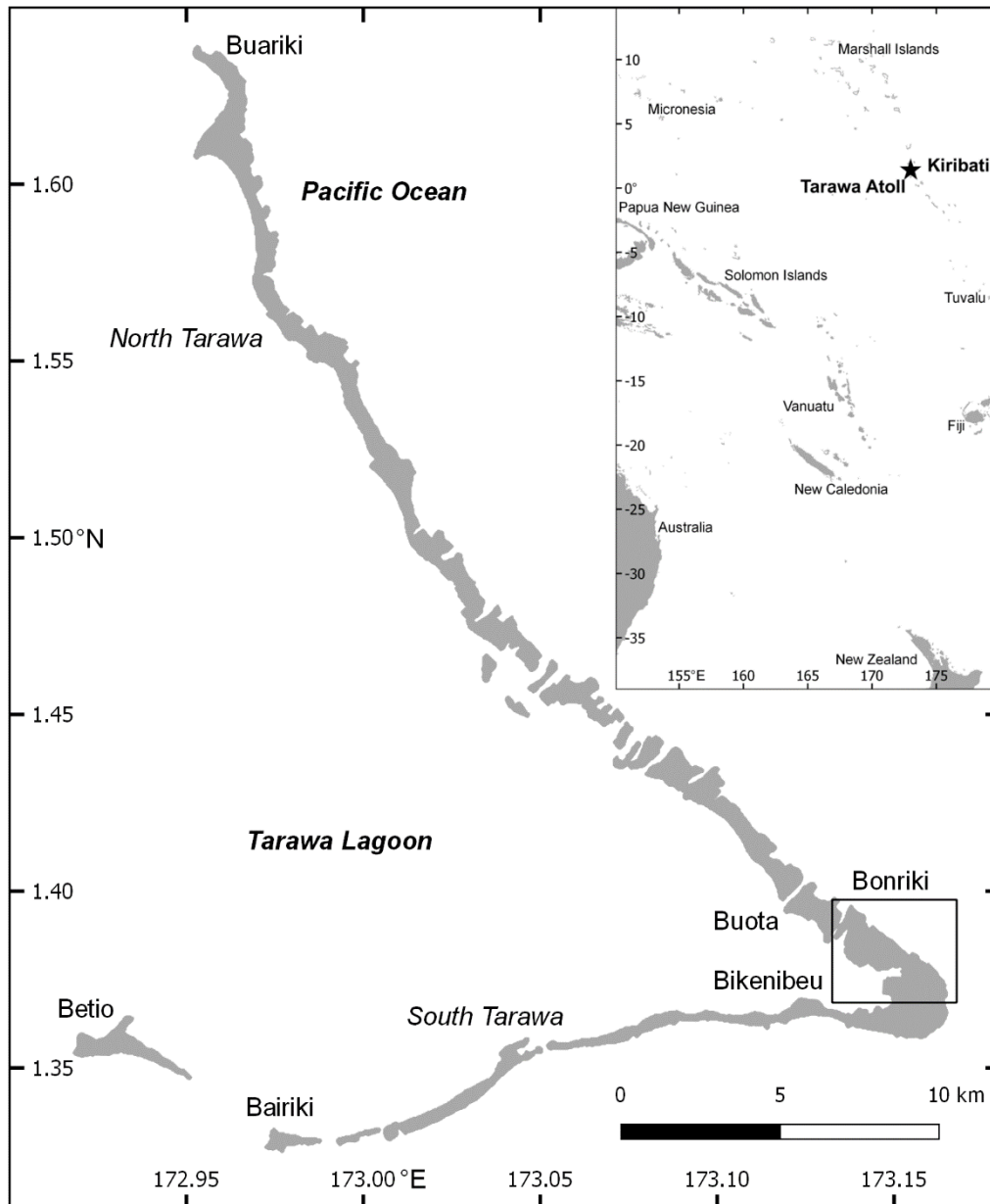
Figure 1. Locality map of Tarawa Atoll and Bonriki Island (taken from Post et al., 2018).
