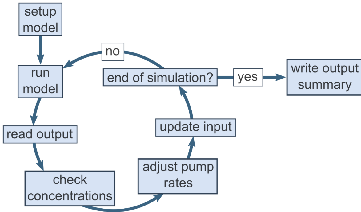
Figure 4. Schematic diagram showing the main program flow used in the script-based approach to evaluate management scenarios. In this study, the loop depicted by the circle was executed 120 times and each model run lasted 3 months, bringing the total simulation period to 30 years.
