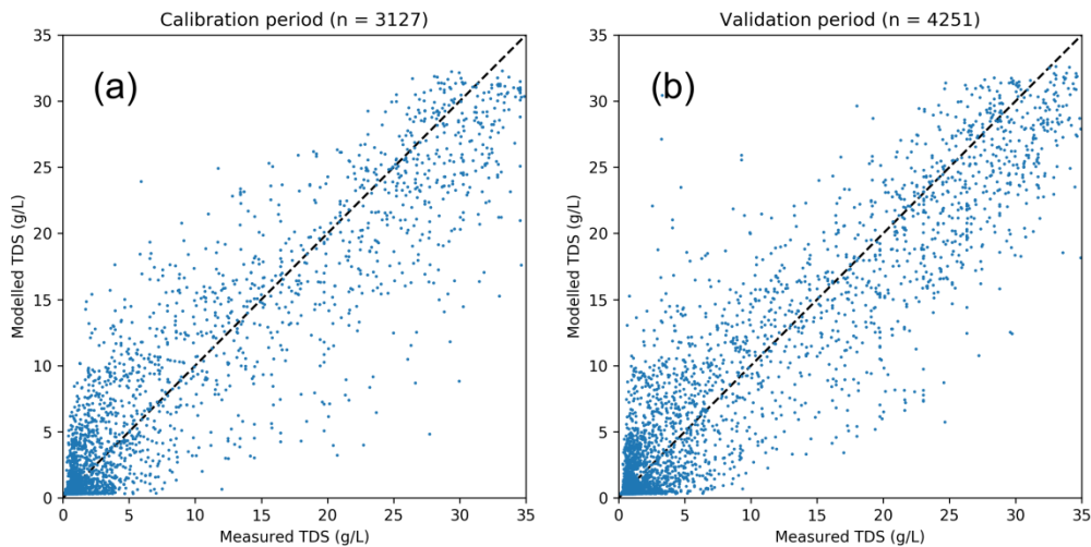
Figure 7. Modelled versus observed concentrations for (a) the calibration period 1997 – 2014 and (b) the validation period 1948 – 1996.
