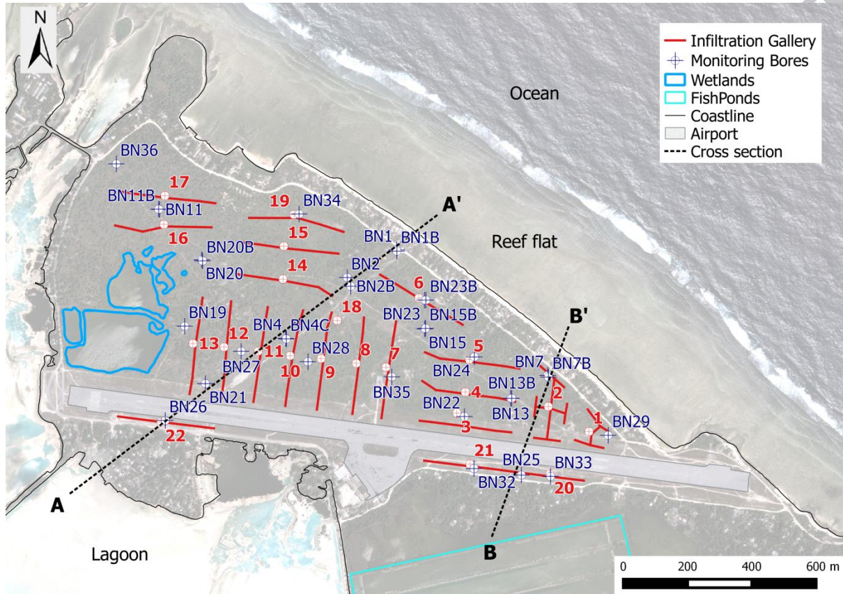
Figure 2. Map showing the Bonriki Water Reserve, horizontal collector wells (known as infiltration galleries) with pumping station structures located in the centre of each gallery, and monitoring bore locations. The blue lines in the western region of the island indicate the location of inland lakes. AA' and BB' identify cross sections shown in later figures. The elevation of the terrain where galleries 9 – 13 are located is lower by about 1 m on average compared to where the other galleries north of the runway are. See Figure 1 for map location.
