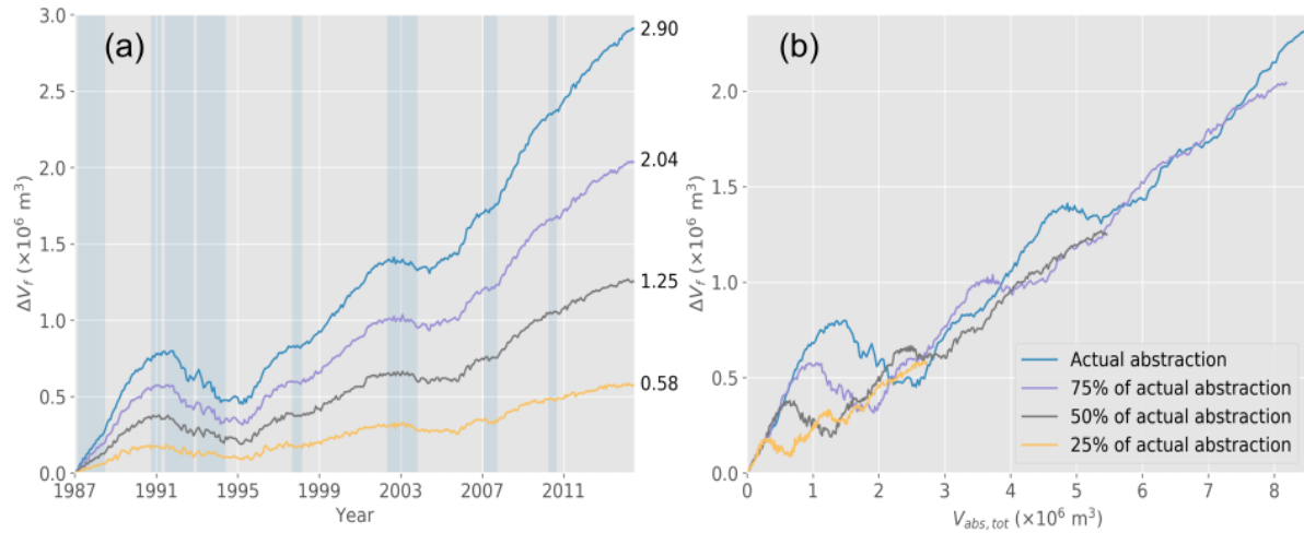
Figure 12. Trends in \Delta V_f for different abstraction rates, plotted as a function of (a) time and (b) V_{\text{abs,tot}} . The percentages shown in the legend represent the fraction of abstraction (relative to the calibrated model) used in modified-pumping simulations. Note vertical scale differences. The blue bars in the left figure indicate periods when R_{12} > 75\% .
