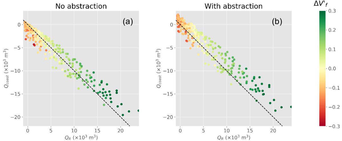
Figure 13. Graphs showing the net flow rate of groundwater across the coastal boundary ( Q_{\text{coast}} ) plotted against the net volumetric recharge rate ( Q_R ) for the model (a) without abstraction and (b) with abstraction. Marker symbol colours indicate \Delta V'_f ( \times 10^6 \text{ m}^3 ). Positive values of Q_{\text{coast}} indicate that seawater inflows exceed SGD, and positive values of \Delta V'_f represent periods of lens growth.
