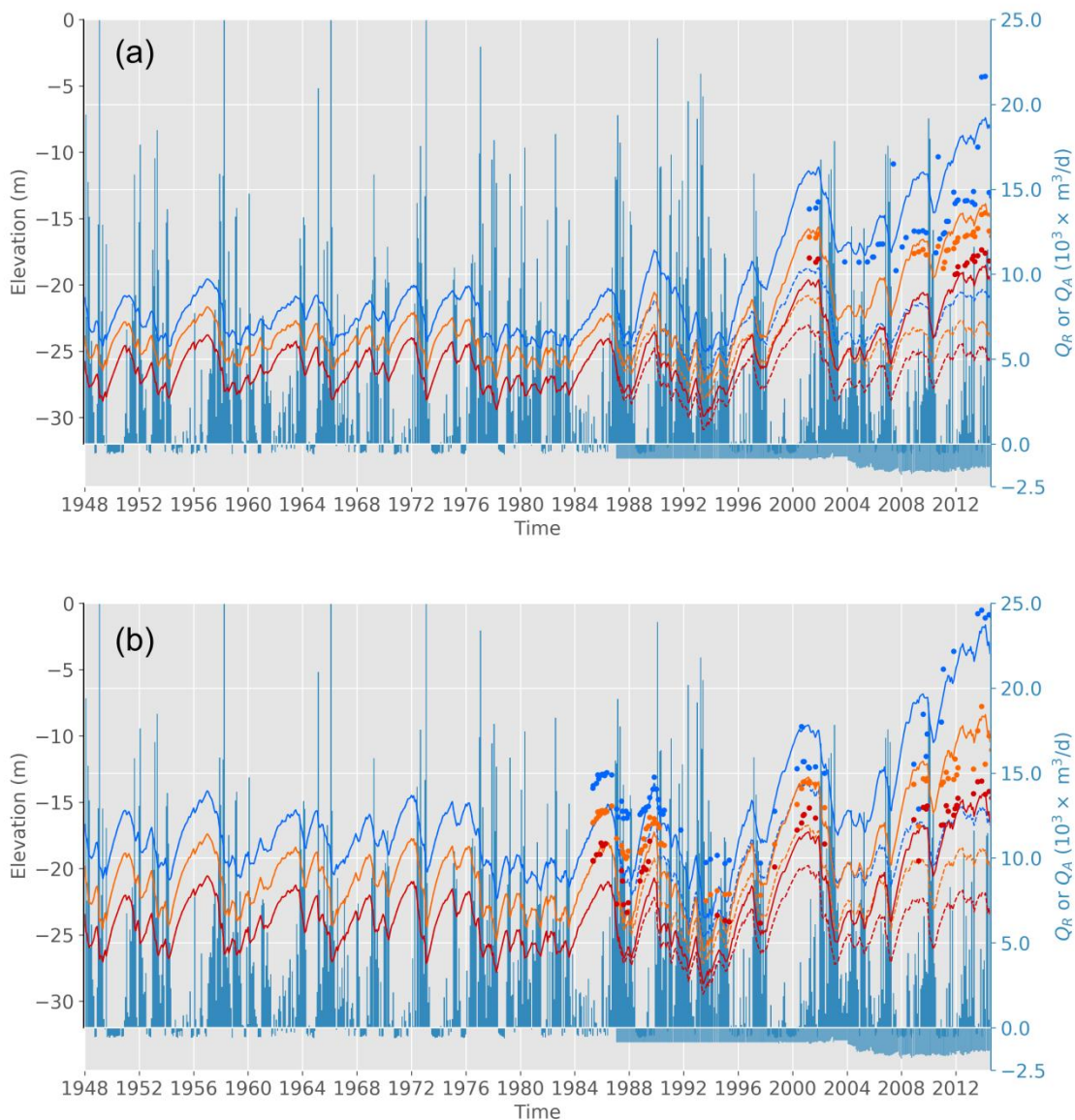
Figure 8. Comparison of the modelled (solid lines) and measurement-based (points) vertical position of EC contour lines of 2.5, 10 and 25 mS/cm (blue, orange and red, TDS values of 1.8, 7.2 and 18 g/L, respectively) at (a) BN27 on cross section A-A' and (b) BN13 on cross
