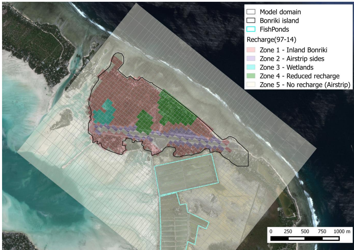
Figure 6. Map showing the outline of the finite-difference grid and the distribution of recharge zones across Bonriki Island.
