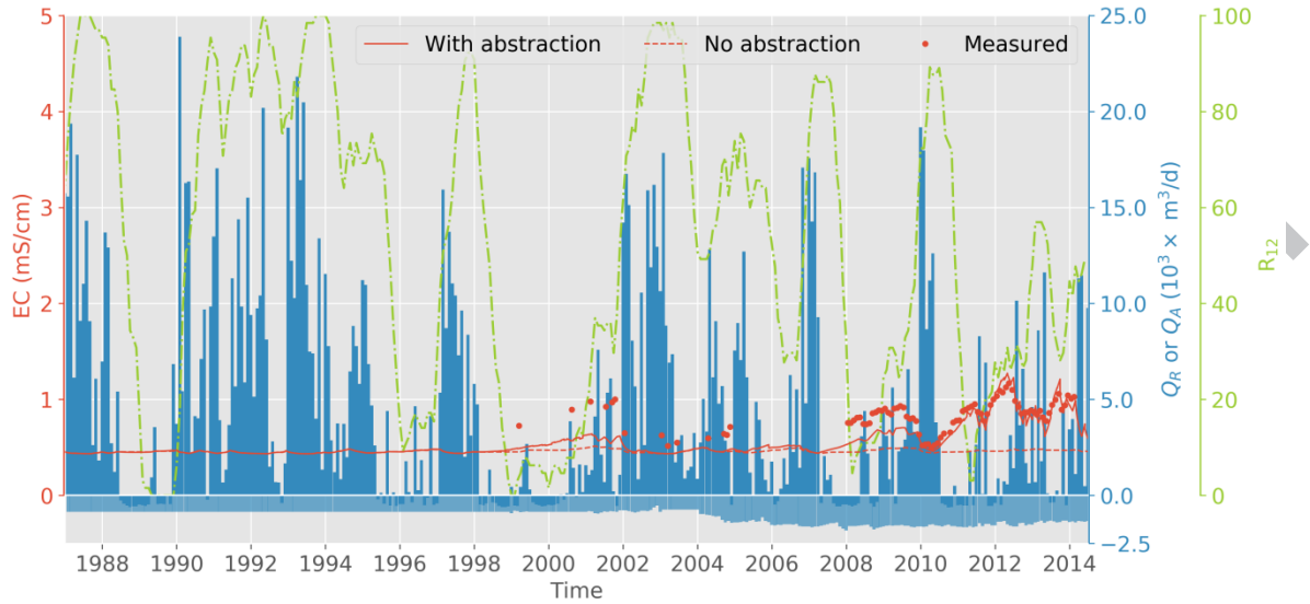
Figure 9. Comparison of computed and measured EC values of the pumped water at the trunk main during January 1987 to June 2014. The solid and dashed red lines represent model scenarios with and without abstraction, respectively. The volumetric recharge and abstraction rates are plotted as dark blue and light blue bars, respectively. The green line represents the 12-month rainfall ranking ( R_{12} ; see Section 3.4).
