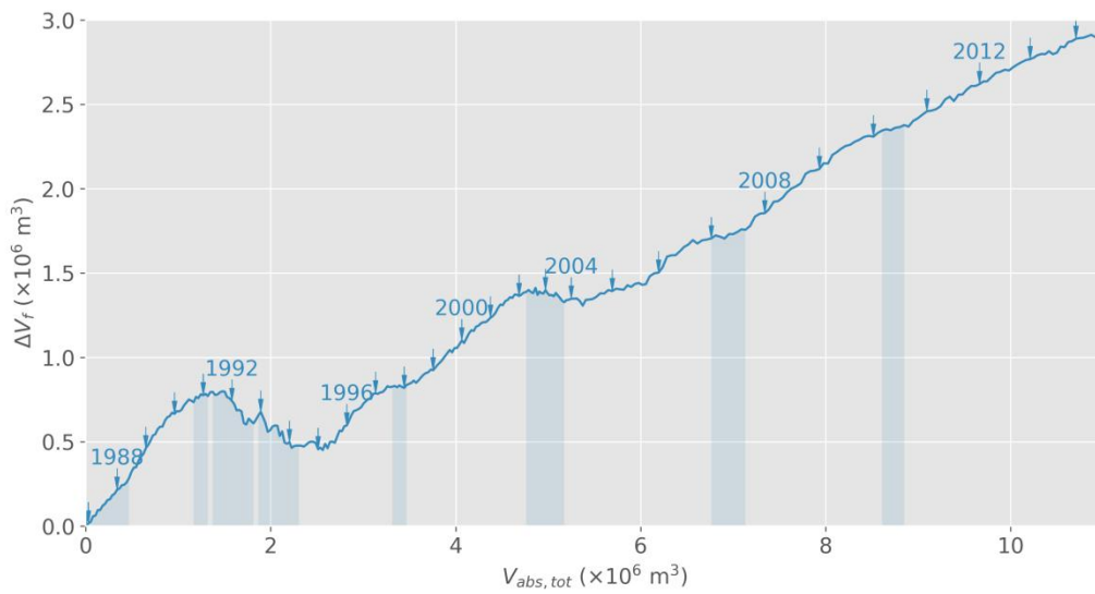
Figure 11. Graph showing the pumping-induced depletion of the lens ( \Delta V_f ) plotted against the total volume of pumped groundwater ( V_{abs,tot} ). The blue bars in the figure indicate periods when R_{12} > 75\% , i.e., periods of very high rainfall. The blue arrows mark the start of years.
