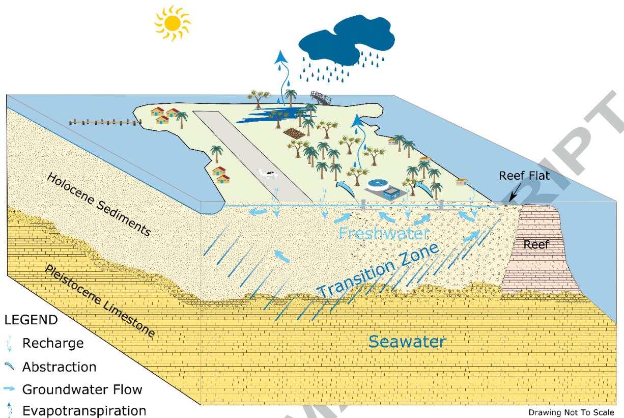
Figure 5. Conceptual three-dimensional block diagram of the Bonriki groundwater system, modified from Bosserelle et al. (2015). Coarser sediments encountered in the region closest to the ocean (right-hand) boundary are illustrated by the pattern change within the Holocene layer. Symbols courtesy of the Integration and Application Network, University of Maryland Center for Environmental Science ( ian.umces.edu/symbols/ ).
