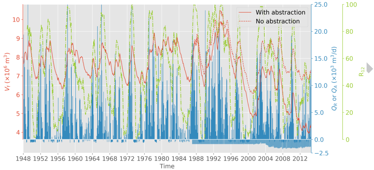
Figure 10. Simulated freshwater volume ( V_f ) during the period January 1948 – June 2014. The solid red line represents the model scenario with abstraction, the dashed line is for the model with no pumping. The volumetric recharge and abstraction rates are plotted as dark blue and light blue bars, respectively. The green line represents the 12-month rainfall ranking ( R_{12} ).
