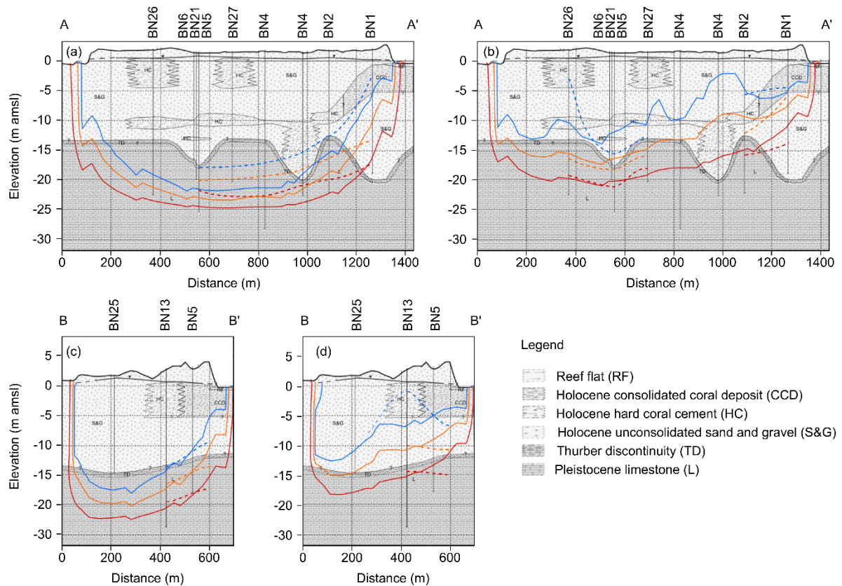
Figure 3. Cross sections showing the lithology, water table elevation and freshwater lens geometry for (a) May 1985 along profile line A-A', (b) June 2014 along profile line A-A', (c) May 1985 along profile line B-B', (d) June 2014 along profile line B-B'. Cross section locations are shown in Figure 2. The dashed lines represent electrical conductivity (EC) contours of 2.5, 10 and 25 mS/cm (blue, orange and red colours, respectively) based on interpolation of field measurements. Solid lines are obtained from the numerical model (see Section 3). The EC contour values correspond to a TDS of 1.8, 7.2 and 18 g/L, respectively, and were adopted for consistency with previous publications (e.g., Falkland and Woodroffe, 2004).
