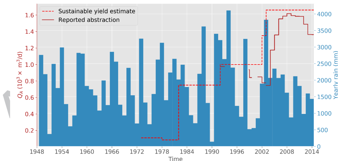
Figure 4. Overview of pumping rates and published sustainable yield estimates for the Bonriki lens, according to Mather (1973), AGDHC (1982), Falkland (1992), Alam et al. (2002), White et al. (2002), White et al. (2008), and Sinclair et al. (2015). The recorded
