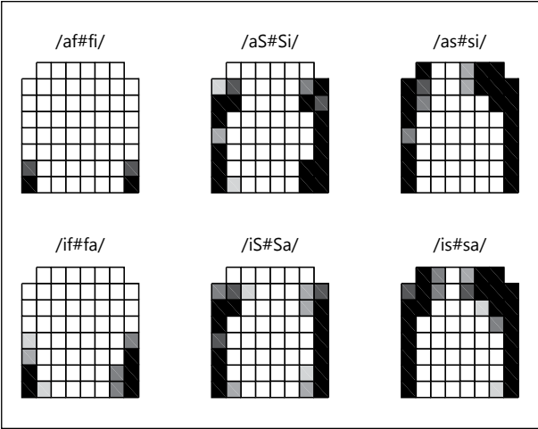
Fig. 8. Palatograms for speaker 9. Shown are the reference patterns for the 3 homorganic control conditions for 2 vowel contexts, unstressed-stressed condition. The reference patterns served as the basis for the by-speaker, by-condition index calculation; see Methods for details. Shading is equivalent to percent average contact over repetitions with black being 100% and white being 0. The anterior is oriented towards the top in each graph.
