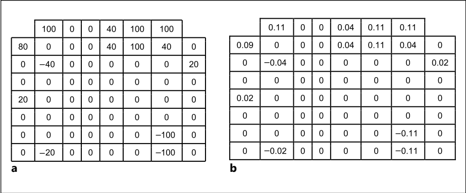
Fig. 9. Illustration of the difference pattern by which each EPG sample was weighted. The difference pattern was created by subtracting – on a by-condition, by-subject, by-electrode basis – the relevant reference conditions from each other (here: /s#s/ – /f#f/, i-a, unstressed-stressed, speaker 9, i.e. the bottom row mid and rightmost palatograms of fig. 8) and dividing each electrode’s difference value by the sum of the absolute values of all the electrodes in the raw difference pattern; see Methods for more detail. a Raw difference pattern (/ss/ – /ff/). b Normalized difference pattern [(/ss – ff)/Σ abs(difference pattern)].
