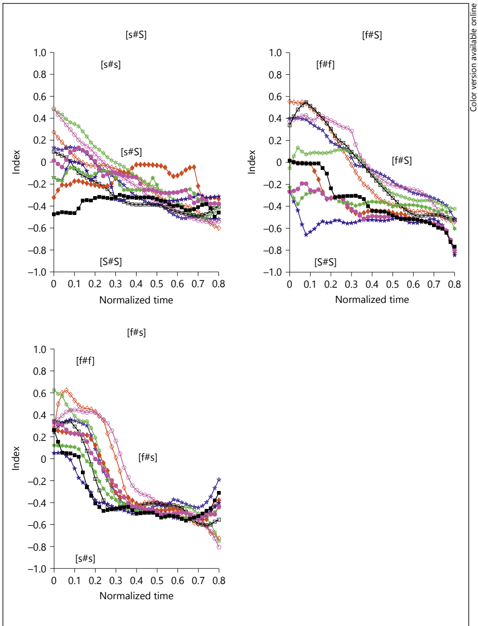
Fig. 7. Spread-normalized EPG and acoustic indices for the same data as presented in figure 4, without the controls. Filled symbols show the EPG index, empty symbols the acoustic index. The indices belonging to the same repetition have the same symbol type and color. The time interval has been cut off at 0.8 for presentation purposes since converging acoustic control indices lead to extremely large spread-normalized values at the edge.
