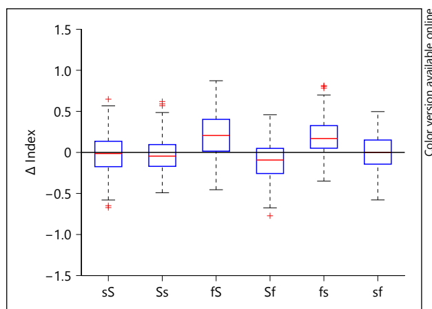
Fig. 3. EPG acoustic \Delta index for all clusters.
