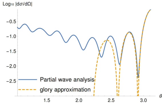
Fig. 10. Differential scattering cross section of a massless scalar wave with frequency \omega = 25 scattered by a skyrmion black hole of CASE I ( \alpha = 0.01 , \beta = 0 and x_h = x_h^{max, \alpha=0.01, \beta=0} = 0.1263 ).
