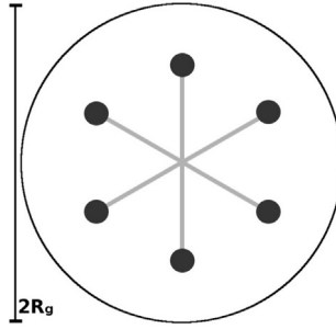
Fig. C.17. Illustration of a state with N_C = 6 quarks attached to a single junction by QCD flux tubes in the case when the length of each string R is smaller than the gravitational radius R_g of the state.
