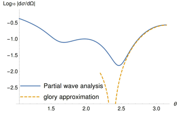
Fig. 9. Differential scattering cross section of a massless scalar wave with frequency \omega = 8 scattered by a skyrmion black hole of CASE I ( \alpha = 0.01 , \beta = 0 and x_h = x_h^{max, \alpha=0.01, \beta=0} = 0.1263 ).
