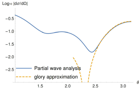
Fig. 11. Differential scattering cross section of a massless scalar wave with frequency \omega = 8 scattered by a skyrmion black hole of CASE II ( \alpha = 0.01 , \beta = 0.5 and x_h = 0.116 ).
