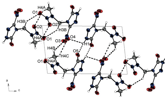
Fig. 4 Unit cell of 1-(3-nitro-1 H -1,2,4-triazol-5-on-4-yl)-2-nitrazopropane ( 1 ) along the b axis. Thermal ellipsoids are drawn at the 50% probability level. Selected hydrogen bonds are shown as black dotted lines.
