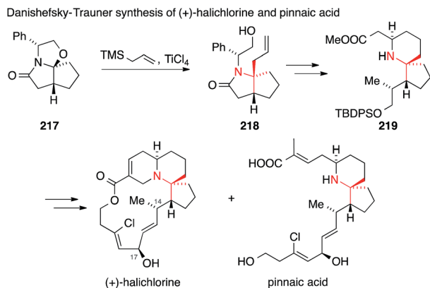
Scheme 48 Synthesis of halichlorine and pinnaic acid by Danishefsky and Trauner (1999). TBDS = tert -butyldiphenylsilyl, TMS = trimethylsilyl.
