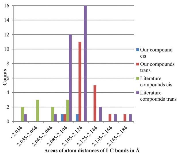
Fig. 8 Statistical distribution of the C-I atom distances of all diiodides discussed here, separated in cis/trans and literature compounds and ours. C_{2}I_2^{18} was excluded because of the very short C-I distance (1.987(3) Å), F_3C^{19} and C_2I_4^{20} are included in the literature trans category. cis Diiodo compounds, which are mostly cyclic, have shorter C-I atom distances than linear ones and those with trans configuration. They are even shorter than the literature value given for the C_{Ar}-I distance (2.095 Å). 21
