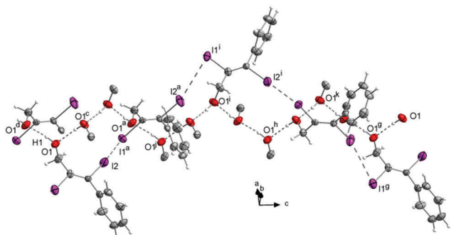
Fig. 11 Crystal structure of 4 . One turn of the helix formed by the I...I halogen bonds (I2 to I1 g ) includes three turns of the helix formed via hydrogen bonds (O1 to O1 l ; O1 l to O1 h ; O1 h to O1 g ) d(\text{O} \cdots \text{H}) = 0.84(2) Å, d(\text{O1} \cdots \text{O1}^g) = 2.693(3) Å, \angle \text{O1} - \text{H1} \cdots \text{O1}^g = 169.6(2)^\circ . Some (I)C=C(I)Ph residues are omitted for clarity. Symmetry codes: (a) (-0.25 + x, 1.25 - y, 0.75 + z) , (c) (1.25 - x, 0.25 + y, 0.25 + z) , (g) (x, y, 3 + z) , (h) (x, y, 2 + z) , (i) (1.5 - x, 1 - y, 1.5 + z) , (j) (x, y, 1 + z) , (k) (1.5 - x, 1 - y, 2.5 + z) . DIAMOND representation, thermal ellipsoids are drawn at 50% probability level.
