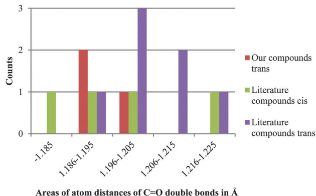
Areas of atom distances of C=O double bonds in Å
