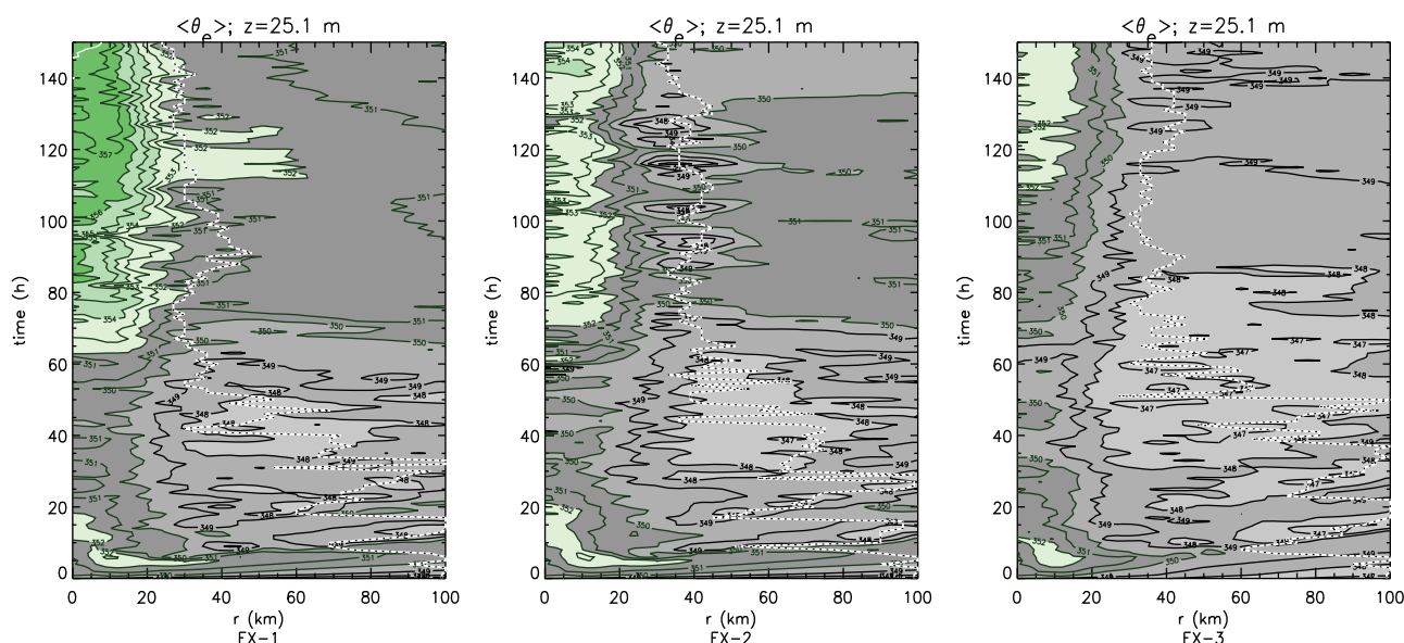
Figure 7. Azimuthally-averaged \langle \theta \rangle at z=25.1 m from (left) EX-1, (middle) EX-2, and (right) EX-3 with contours at 1 K intervals with shading white < 346 K, light gray < 348 K, medium gray < 350 K, dark gray < 352 K, light green < 354 K, medium green < 355 K, dark green > 354 K.
