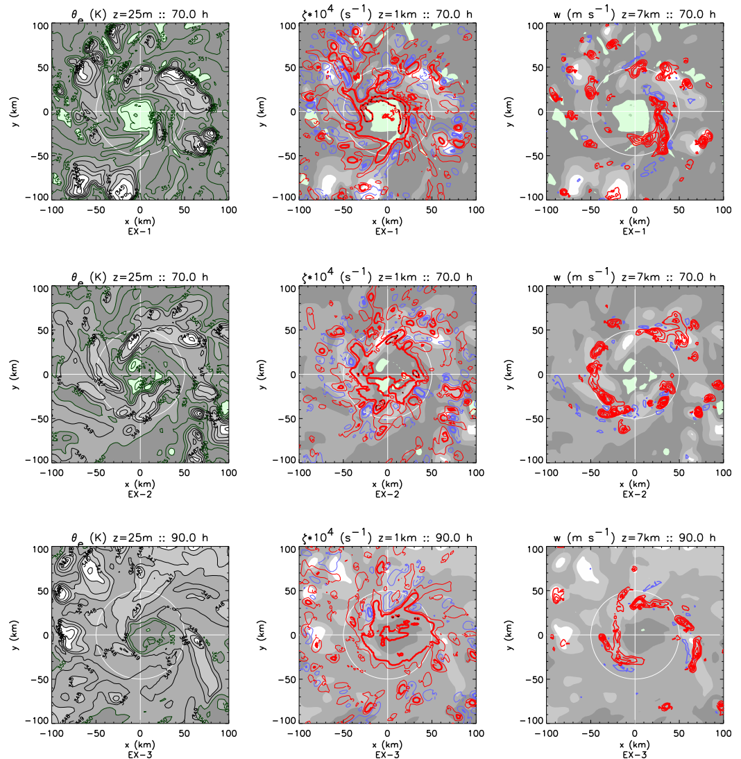
Figure 6. Thermodynamic and dynamic quantities at a moment of rapid intensification from (first row) EX-1, (middle row) EX-2, and (bottom row) EX-3. In the left column, \theta_p at the 25-m level is contoured at 1 K intervals with shading (also shown in the middle and right columns) white < 346 K, light gray < 348 K, medium gray < 350 K, dark gray < 352 K, light green < 354 K, medium green < 356 K, dark green > 358 K. In the middle column, \zeta \times 10^4 is contoured with contours ( s^{-1} ) -10 (thick blue), -3 (blue), 3 (red), 10 (thick red), and 30 (spotted red). In the right column, w is contoured with contours ( m s^{-1} ) -2 and -1 (blue) and 1, 2, 3, 4, and 5 (red).
