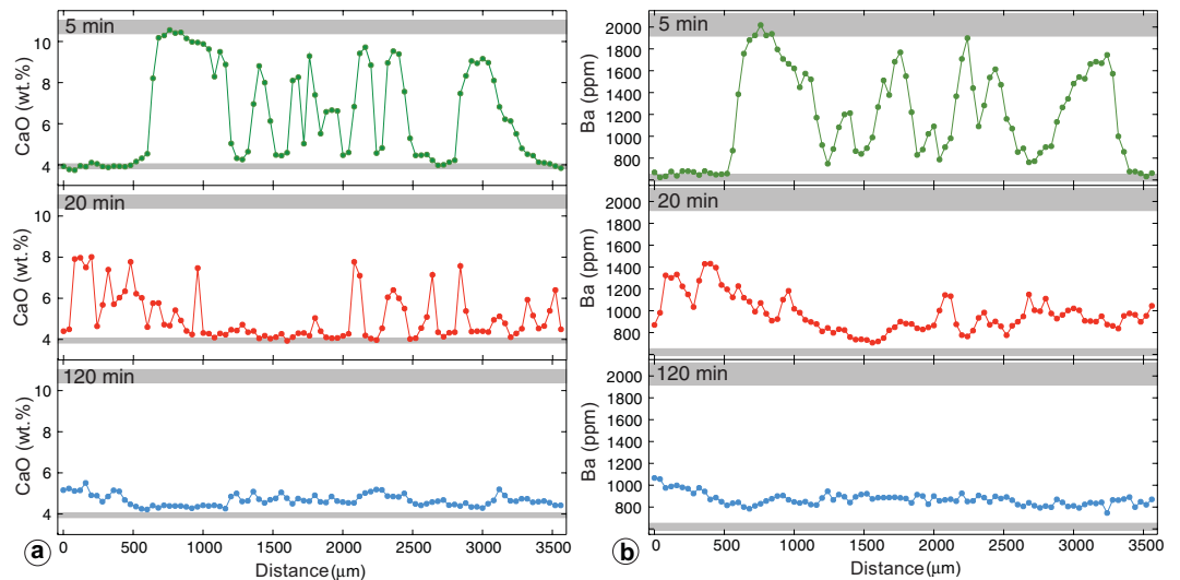
Figure 2. Representative compositional variation of CaO (a) and Ba (b) along the mixing interface (i.e. along the white horizontal lines in Fig. 1b-d) at different mixing times. Concentrations of initial basaltic and phonolitic melts are marked in grey areas including analytical uncertainties as standard deviations.
