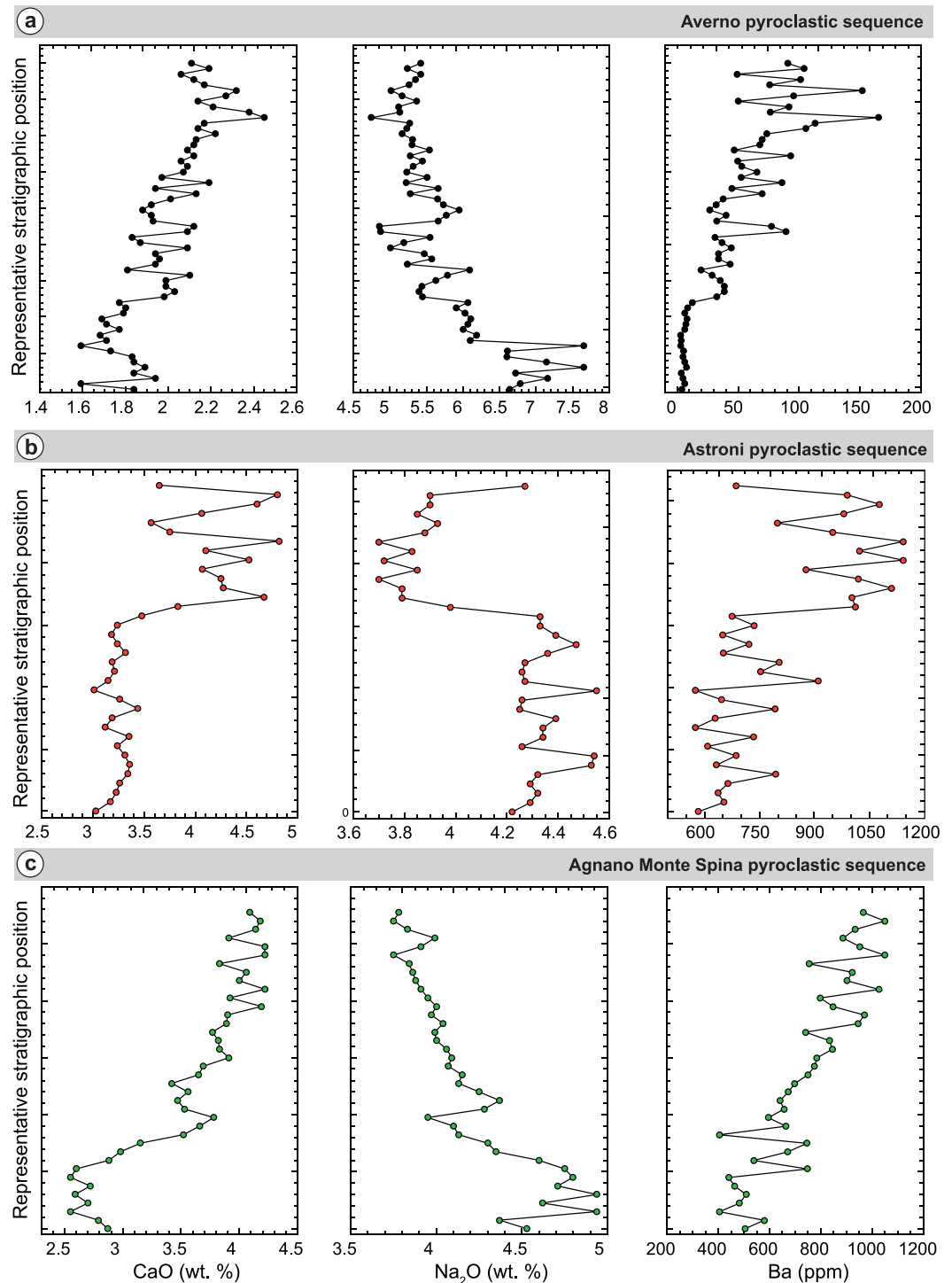
Figure 5. Variation of some representative major and trace elements across the pyroclastic sequences of Averno (a), Astroni (b), and Agnano Monte Spina (c) used to estimate the mixing-to-eruption time with the CVD method. Height of the sequence is ca. 20 m., 16 m. and 15 m. for Averno, Astroni, and Agnano Monte Spina, respectively.
