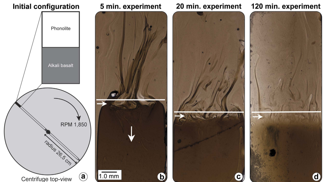
Figure 1. (a) Sketch of the centrifuge used to trigger the injection of the basaltic melt in the phonolite at 1,200 °C. The location and geometry of the experimental sample before the starting of the experiments are also shown. (b–d) Resultant glasses from magma mixing experiments at different mixing time t = 5 min (b), t = 20 min (c) and t = 120 min (d). The vertical white arrow in (b) indicates the direction of motion of the basaltic melt during injection. White lines correspond to the division line of the two melts at t = 0 . The horizontal white arrows in (b–d) indicate the direction in which the analyses were performed.
