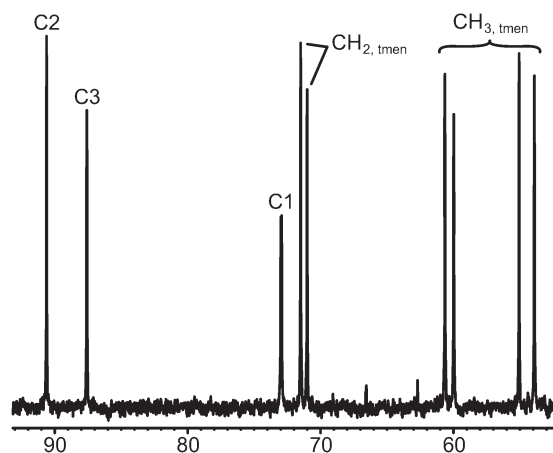
Fig. 3 ^{13}\text{C} NMR spectrum of [\text{ReO}(\text{tmen})(\text{rac-Glyc}2,3\text{H-}2,1\text{PH-}\kappa^3\text{O}^{2,3,\text{p}})] ( 2 ) in \text{D}_2\text{O} measured at 4^\circ\text{C} .
