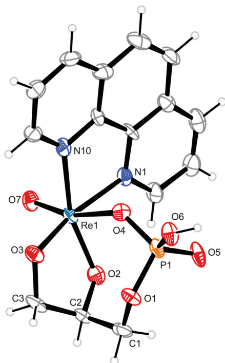
Fig. 4 Structure of [\text{ReO}(\text{phen})(\text{rac-Glyc2,3H-}_2\text{1PH-}\kappa^3\text{O}^{2,3,\text{P}})] ( 3 ) in crystals of the methanol adduct (50% probability ellipsoids). Distances ( \text{\AA} ) and angles ( ^\circ ): from Re1 to: O2 1.917(6), O3 1.957(6), O4 2.102(6), O7 1.690(6), N1 2.129(6), N10 2.158(7); from P1 to: O1 1.583(6), O4 1.527(6), O5 1.490(7), O6 1.558(7); O2–Re1–O3 82.7(3), O2–Re1–O4 88.2(2), O3–Re1–O4 85.5(2), O2–Re1–O7 106.8(3), O3–Re1–O7 103.8(3), N1–Re1–N10 77.7(3); O2–C2–C3–O3 -32.2(9) . Centrosymmetric dimers form via two short hydrogen bonds (O6...O5 i and O6 i ...O5 2.495(8); i –x, –y, –z) in a carbonic-acid-dimer-typical way.
