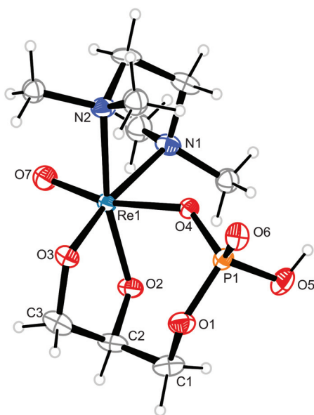
Fig. 2 Molecular structure of [\text{ReO}(\text{tmen})(\text{rac-Glyc}2,3\text{H-}2,1\text{PH-}\kappa^3\text{O}^{2,3,\text{p}})] ( 2 ) in crystals of the dihydrate (50% probability ellipsoids). Distances ( \text{\AA} ) and angles ( ^\circ ): from Re1 to: O2 1.941(3), O3 1.954(3), O4 2.067(3), O7 1.678(3), N1 2.230(4), N2 2.224(4); from P1 to: O1 1.587(3), O4 1.528(3), O5 1.558(3), O6 1.483(3); O2–Re1–O3 82.26(13), O2–Re1–O4 85.24(12), O3–Re1–O4 88.40(12), O2–Re1–O7 106.18(14), O3–Re1–O7 101.51(14), N1–Re1–N2 81.69(15); O2–C2–C3–O3: -37.9(5) . The O5H group forms a short hydrogen bond (O5...O91 2.522(5)) to one of the water molecules.
