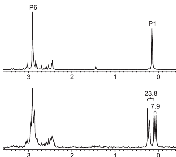
Fig. 1 The 31 P{ 1 H} NMR spectrum (top) and the 31 P NMR spectrum (bottom) of the blue residue obtained by evaporating the reaction solution containing the product complex anion [ReO(tmen)(Fru 2 ,3H -2 ,1,6P 2 H 2 -κ 3 O 2,3,P1 )] - ( 1 ) in methanol-d 4 with 31 P– 1 H NMR coupling constants ( 3 J P,H /Hz).
