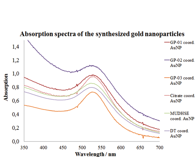
Fig. 3 UV/Vis spectra of the synthesized nanoparticles.
