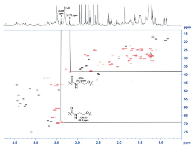
Fig. 4 HSQC-spectra of the GP-01 coordinated AuNP; red = co-ordinated ligand, black = free glycopeptides.
