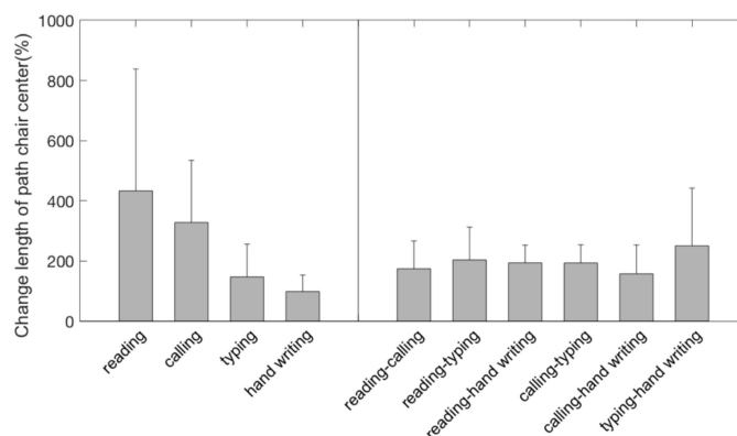
Figure 3. Relative increase in path length of the chair center for sitting on the dynamic chair compared to the static chair for the different tasks and task transitions.
