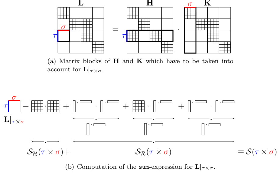
FIGURE 3. Illustration why a block \mathbf{L}|_{\tau \times \sigma} on the coarsest level of the target \mathcal{H} -matrix can be represented as a sum-expression \mathcal{S}(\tau, \sigma) .
