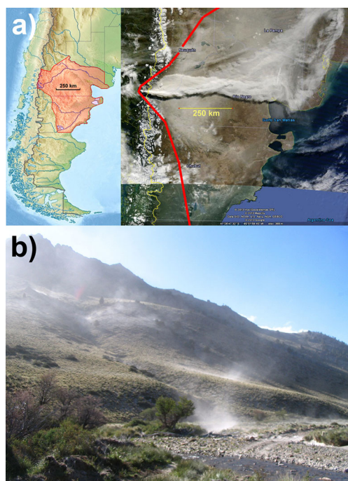
Fig. 1 a Distribution of tephra deposited from the Puyehue–Cordon Caulle volcanic eruption, showing the Moderate Resolution Imaging Spectroradiometer image of 13 June 2011, http://earthobservatory.nasa.gov . The red line marks the limit of deposition, principally in the Provinces of Neuquen, Rio Negro, and Chubut. b Ecotonal landscape in the Patagonian study area. Although known for commonly strong eolic conditions, this was a “calm day without westerlies: This turbulence is due to daily thermal wind patterns which shift ashes in any direction (color figure online)
