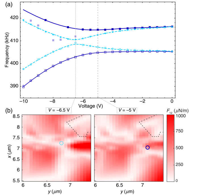
FIG. 2. (a) Mode frequencies as a function of voltage applied over the two gates. Data points represented by light blue circles are taken at the position indicated by the dashed circle drawn in the left panel of (b), while the dark blue squares correspond to data taken at the position of the solid circle drawn in the right panel. The curves are fits of Eq. (2) to the data. Gray points are data points not used in the fits. Both sets of data show avoided crossings, with different splittings due to different coupling strengths. (b) Spatial maps of the measured coupling term F_{12} for V = -6.5 V (left) and V = -5 V (right). The dashed black line indicates the position of the nearest gate electrode.
