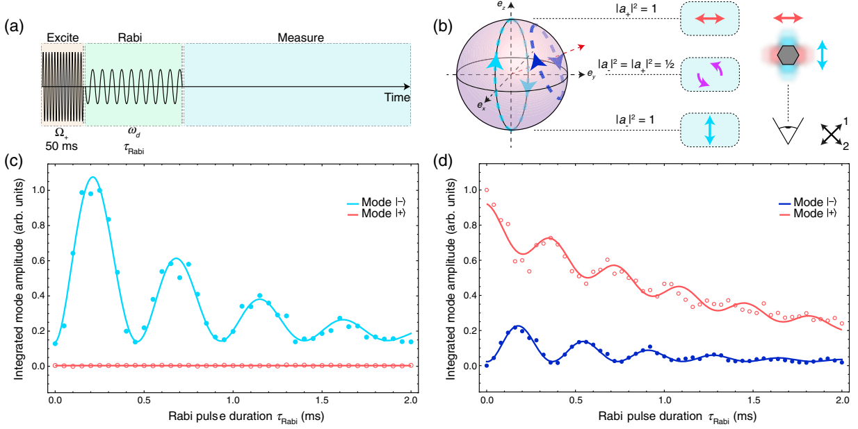
FIG. 4. (a) Schematic of Rabi pulsing scheme. (b) Bloch sphere representation of Rabi oscillations. Light blue (vertical) arrow indicates Rabi oscillations for \delta_d = 0 ; dark blue (tilted) arrow indicates Rabi oscillations for \delta_d \neq 0 . Boxed arrows on the right side schematically indicate NW in the plane for different population distributions. Right panel illustrates approximate oscillation directions of the |+\rangle and |-\rangle modes with respect to the optical axis of the detector and the oscillation directions of the original modes. (c) Power spectral densities of both modes as a function of Rabi pulse duration. Points indicate measured data; solid lines are fits to the data. The fit for mode |-\rangle returns a Rabi frequency of 1.9 kHz ( \Delta\Omega/2\pi = 10.9 kHz). Displacement of mode |+\rangle is undetectable due to misalignment of this mode with respect to the optical axis of the detector. (d) Similar to (c) but now for \delta_d \neq 0 . Fits yield Rabi frequencies of 2.8 kHz (mode |-\rangle ) and 3.0 kHz (mode |+\rangle ) ( \Delta\Omega/2\pi = 12.1 kHz). Note that the offset in the measured Rabi oscillations is due to thermal excitation of the mode.
