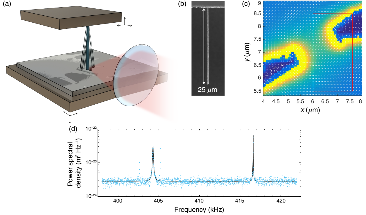
FIG. 1. (a) Overview of the experimental setup. (b) SEM of the NW used in this work. (c) Simulated electric field of the gate electrodes with the tip of the NW placed at a height of 70 nm above the sample surface. The arrows indicate the direction of the field, while the magnitude is encoded in color scale. The red rectangle indicates the region of the sample measured in the remainder of this work. (d) Interferometric measurement of the power spectral density of the two fundamental flexural modes of the NW taken with a tip-sample distance of 70 nm.
