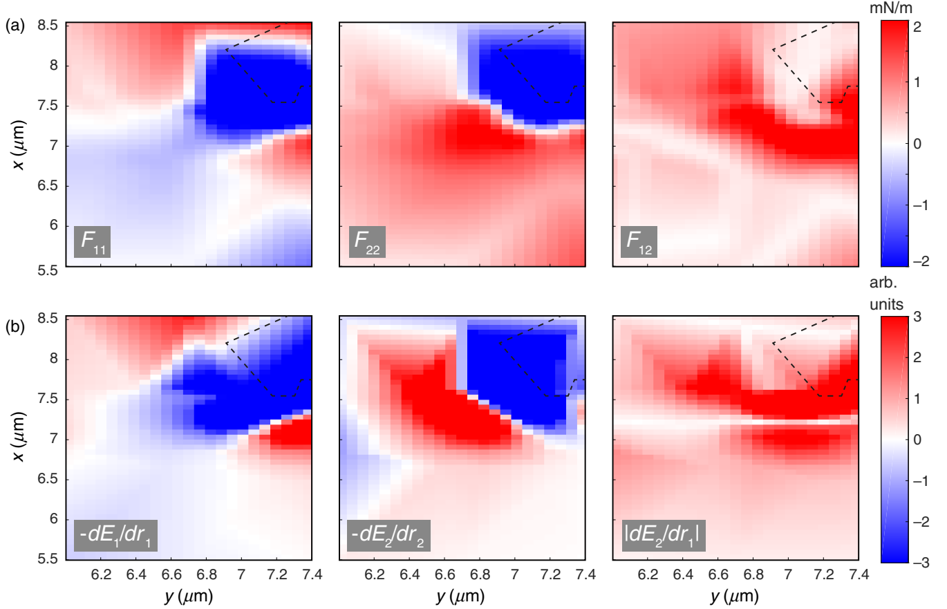
FIG. 3. (a) Spatial maps of the experimentally determined force derivatives F_{11} (left), F_{22} (middle), and F_{12} (right). (b) Simulated derivatives of the electric field -dE_1/dr_1 (left), -dE_2/dr_2 (middle), and |dE_2/dr_1| (right). For all plots V = -10 V.
