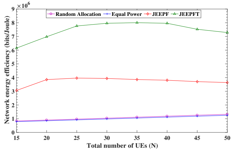
Figure 3.7: EE of different algorithms versus total number of UEs, N .
