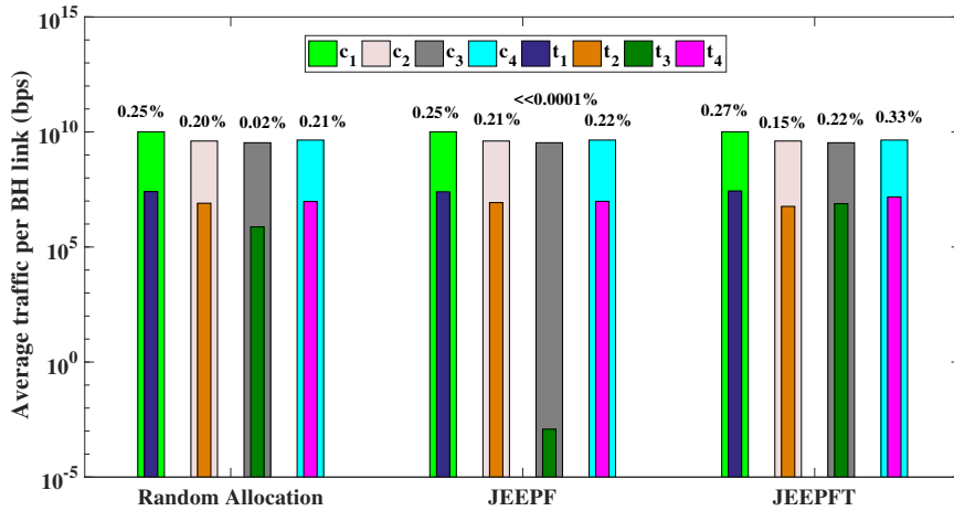
Figure 3.5: Average BH link utilization for different EE algorithms, N=50 UEs.
