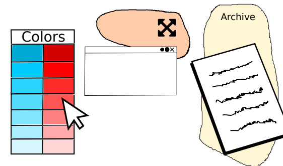
Figure 5: Actions can not only apply to digital documents but also to windows, pointers, or physical objects. For example, the user can change the color of the mouse cursor by clicking into a custom-drawn palette. Windows may be maximized by dragging them into an action region. Placing a paper document on a certain region scans it and archives a digital copy.
