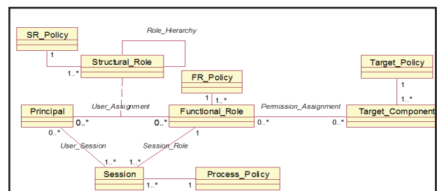
Figure 3: Policy-driven RBAC schema [6].
