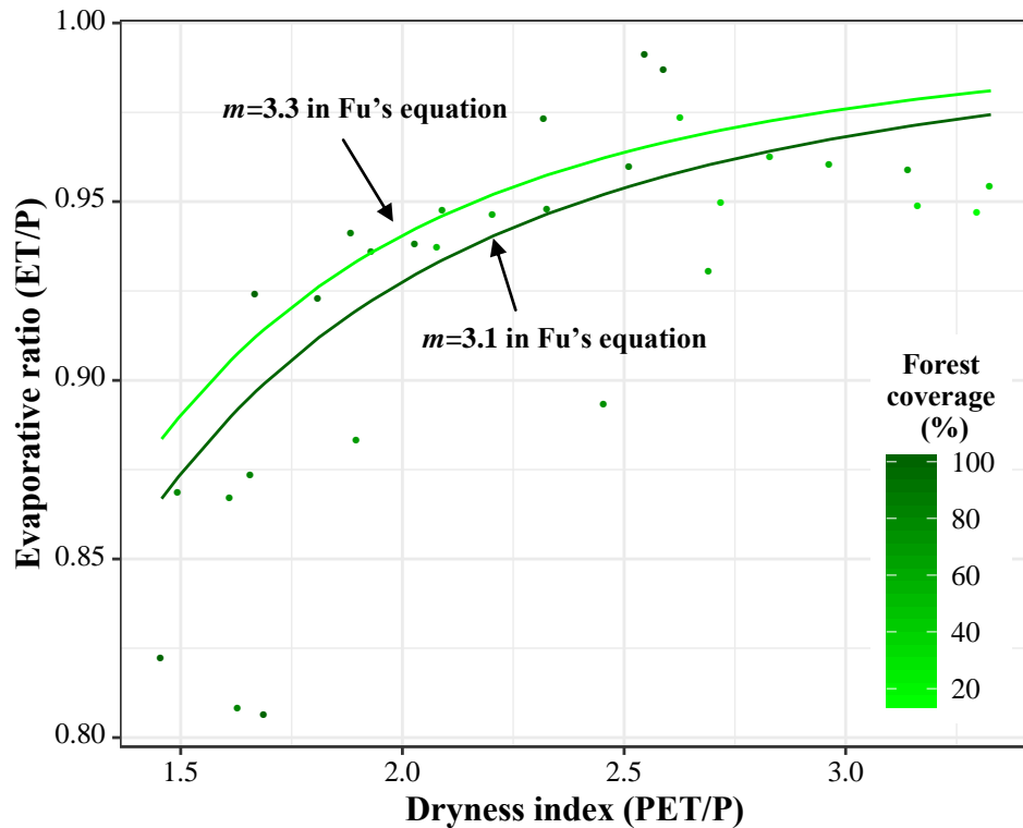
Figure 2 Long-term (1970 to 2015) annual average dryness index (PET/P, the ratio of potential evapotranspiration to precipitation) against evaporative ratio (ET/P, the ratio of evapotranspiration to precipitation) for each catchment. The dark green and light green lines are the best fitted Budyko curves with Fu's equation using catchment parameter m for forest dominant and non-forest dominant catchments, respectively.
