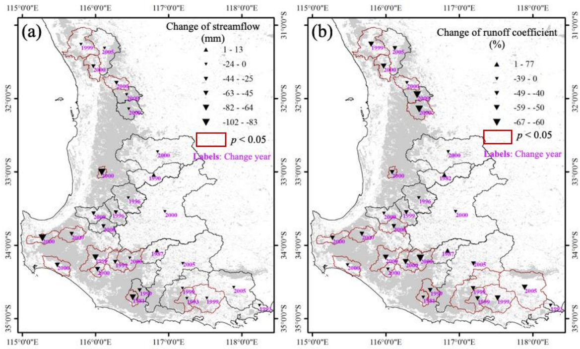
Figure 4 Change of (a) streamflow and (b) runoff coefficient from the pre-change period to the post-change period. Red boundary means that a significant ( p < 0.05 ) breakpoint was found in the catchment from 1970 to 2015.
