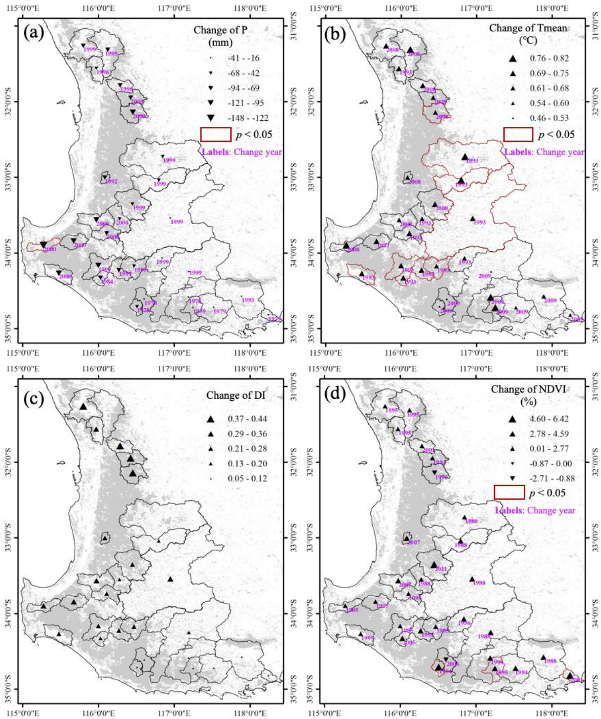
Figure 3 Spatial changes of (a) annual precipitation (P), (b) annual mean temperature (Tmean), (c) annual dryness index (DI) and (d) annual mean normalized difference vegetation index (NDVI) between the pre-change period and the post-change period of each variable for each catchment. The red boundary means that a significant ( p < 0.05 ) breakpoint was found in the catchment from 1970 to 2015, while labels were the detected change year.
