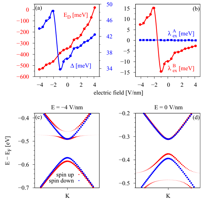
FIG. 8. Influence of the electric field on the proximity-induced parameters for the graphene/hBN/Co structure for two hBN layers, using the minimal p_z model at the K point. Dependence of the (a) Dirac energy E_D and the proximity gap \Delta and (b) the exchange parameters \lambda_{\text{ex}}^A and \lambda_{\text{ex}}^B on the applied transverse electric field. (c) and (d) The calculated spin-resolved band structure projected on the graphene states in the vicinity of the Dirac point for two different field strengths, illustrating the reversal of the valence spin states at the K point.
