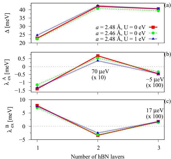
FIG. 13. Influence of the number of hBN layers on the proximity-induced parameters for the graphene/hBN/Ni structure, using the p_z model at the K point. Dependence of (a) the proximity gap \Delta , (b) the exchange parameters \lambda_{\text{ex}}^A , and (c) \lambda_{\text{ex}}^B on the number of hBN layers for different lattice constants or an additional Hubbard parameter of U = 1.0 eV. Parameter values for two (three) layers of hBN were increased by a factor of 10 (100) for better visualization.
