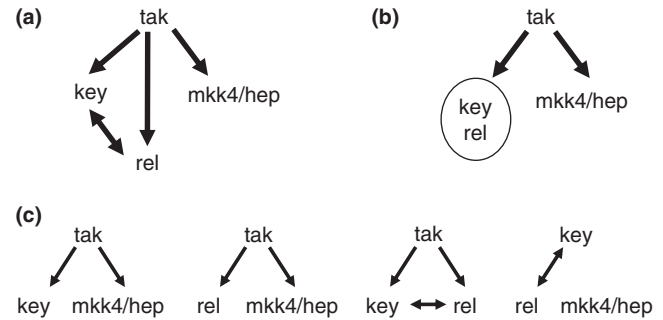
Fig. 5. Results on Drosophila data set. Plot (a) shows the inferred quasi-order, which is the same for all inference methods and agrees with the biological knowledge of this pathway. Plot (b) shows the result after merging two genes with undistinguishable profiles into a single node and removing shortcuts. Plot (c) enumerates the four triple models inferred, which all perfectly match the true structure.
