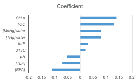
Figure 13. Highly influential predictor variables (VIP scores >1.0) from our PLS analysis of PLSma model to predict Hg contents (THg and MeHg concentrations, %MeHg) in macroinvertebrates, explained with regression model coefficients (coefficient values: >0 for positive correlation; <0 for negative correlation): Chl a =Chlorophyll a in \text{mg m}^{-3} ; \text{d}13\text{C}=\delta^{13}\text{C} ; totP=total phosphorous in \mu\text{g L}^{-1} ; TOC=total organic carbon in \text{mg L}^{-1} ; [TLP]=log-transformed concentration of total lipids ( \text{mg lipids g}^{-1} sample); [BFA]=log-transformed concentration of bacterial fatty acids; [\text{MeHg}]_{\text{water}} =log-transformed aqueous MeHg concentration; [\text{THg}]_{\text{water}} =log-transformed aqueous total Hg concentration.
