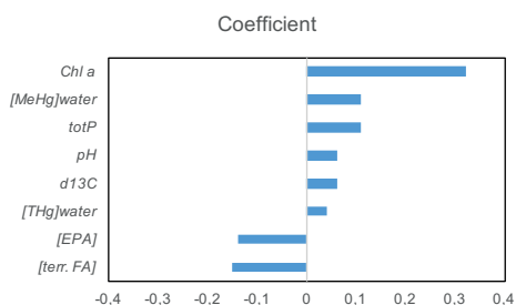
Figure 12. Highly influential predictor variables (VIP scores >1.0) from our PLS analysis of PLSpk model to predict Hg contents (THg and MeHg concentrations, %MeHg) in plankton, explained with regression model coefficients (coefficient values: >0 for positive correlation; <0 for negative correlation): Chl a =Chlorophyll a in mg\ m^{-3} ; d13C= \delta^{13}C ; totP=total phosphorous in \mu g\ L^{-1} ; [EPA]=log-transformed concentration of eicosapentaenoic acid; [MeHg] water =log-transformed aqueous MeHg concentration; [THg] water =log-transformed aqueous total Hg concentration; [terr. FA]=log-transformed concentration of terrestrial fatty acids.
