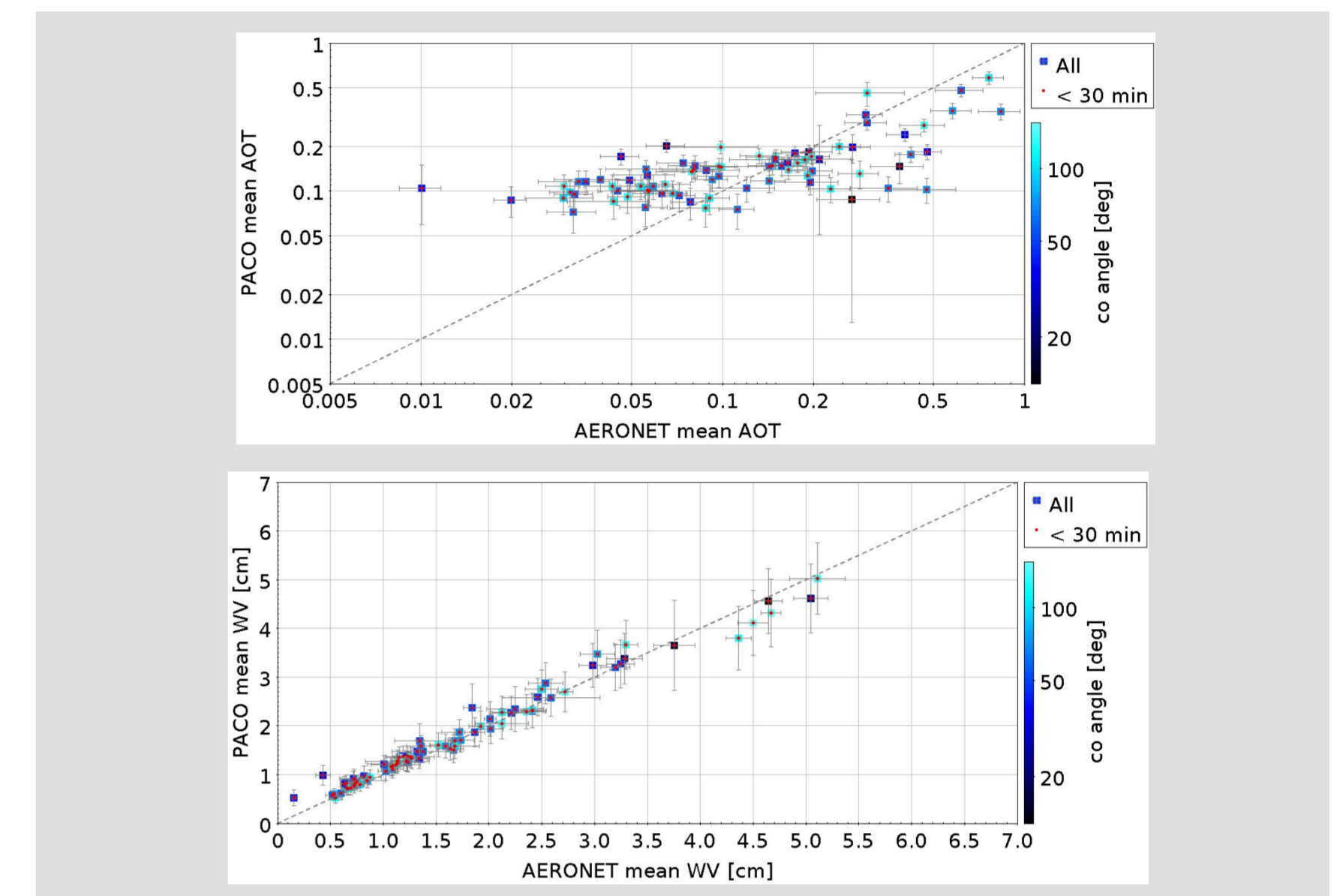
Fig. 1: Scattered plots of the AOT (top) and WV (bottom) of AERONET versus PACO versus the co-location angle (color z-axis) for all final scenes (filled squares) and those with a time difference of 30 min of co-location time (filled red circles).
