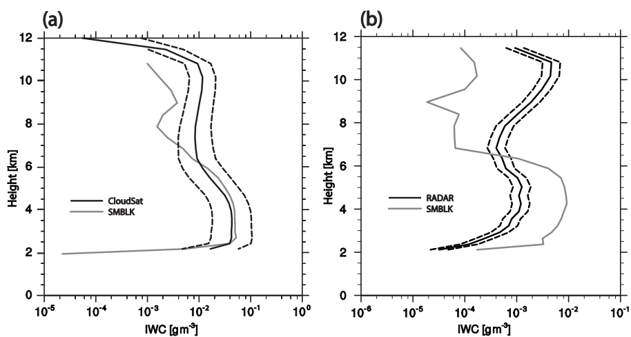
Fig. 8. (a) Spatially averaged vertical profiles of IWC retrieved from cloud radar and the model run SMBLK along the CloudSat satellite overpass on 4 April, 12:30 UTC. (b) Similar to (a), but for the time averaged radar observations and model data at the TROPOS site in Leipzig (51.3 ° N, 12.3 ° E). Absolute values are depicted by full lines, while dashed lines mark the averaged measurement uncertainty of cloud radar retrievals.
