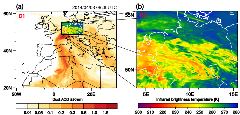
Fig. 1. (a) Model simulation domain D1 with 14km grid spacing showing dust AOD fields by COSMO-MUSCAT. (b) Inner model domain D2 with 2.8 km grid spacing showing simulated infrared brightness temperatures of a COSMO-MUSCAT run with interactive dust effects on cloud microphysics.
