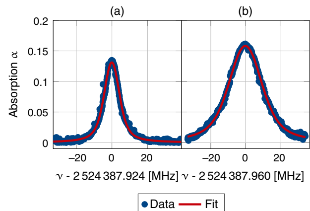
Fig. 6. Absorption spectra of methanol for the observed E2 transition at (a) 0.4 mbar and (b) 0.85 mbar nominal pressure, respectively. The fitted Voigt profile is shown in red.
