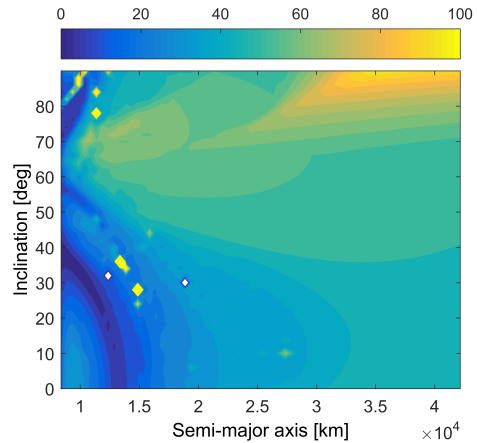
Figure 4. Area-to-mass times reflectivity coefficient [\text{m}^2/\text{kg}] to de-orbit from a 0.2 eccentricity orbit and \Omega_0 = 0 degrees with sail passive mode strategy.
