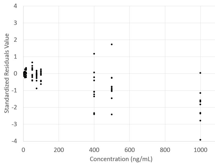
(b) Residuals with a non-normal distribution according to the CVM test
