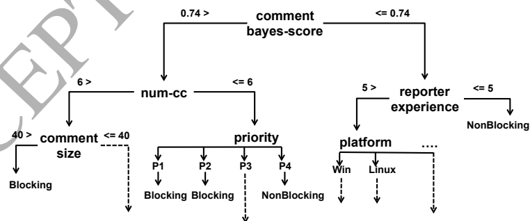
Figure 2: Example of a Decision Tree
