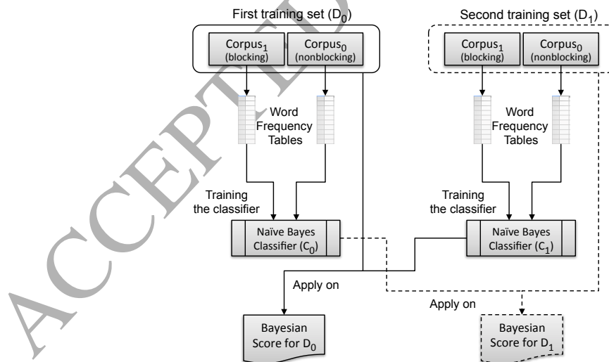
Figure 1: Converting textual factor into Bayesian-score
