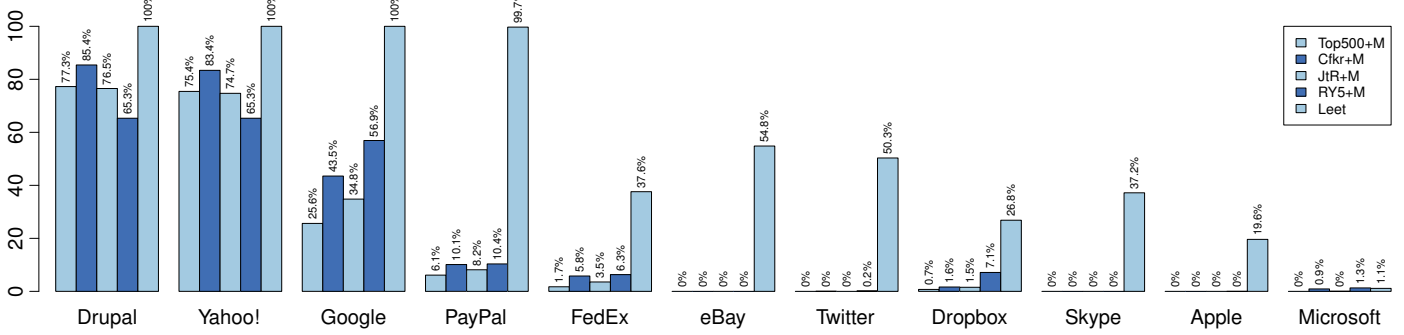
Fig. 8. Comparison between services assigning decent scores to our mangled and leet dictionaries (Microsoft is represented by its latest checker)
