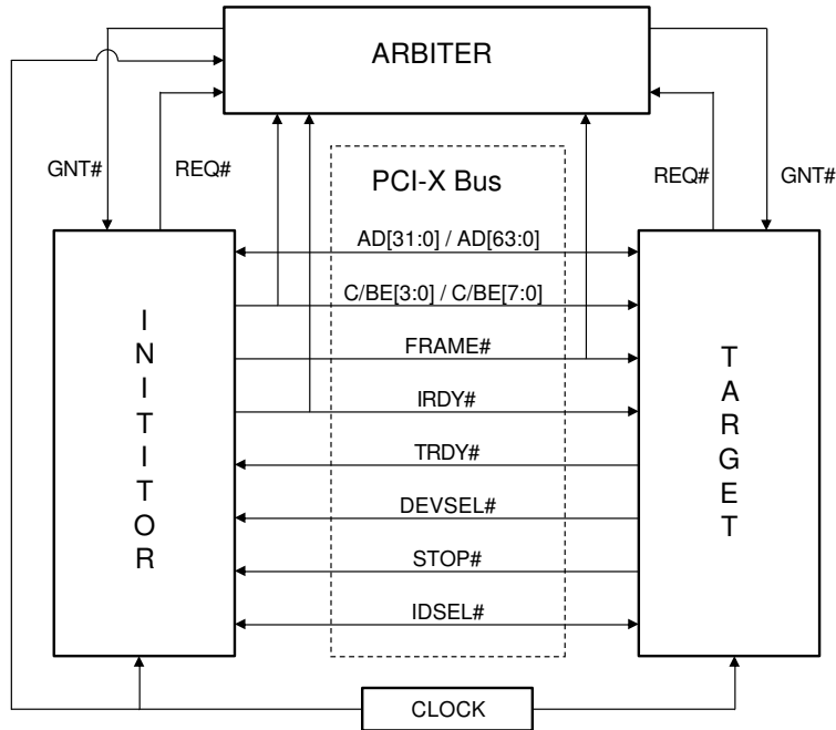
Fig. 5. General Architecture of PCI-X.
