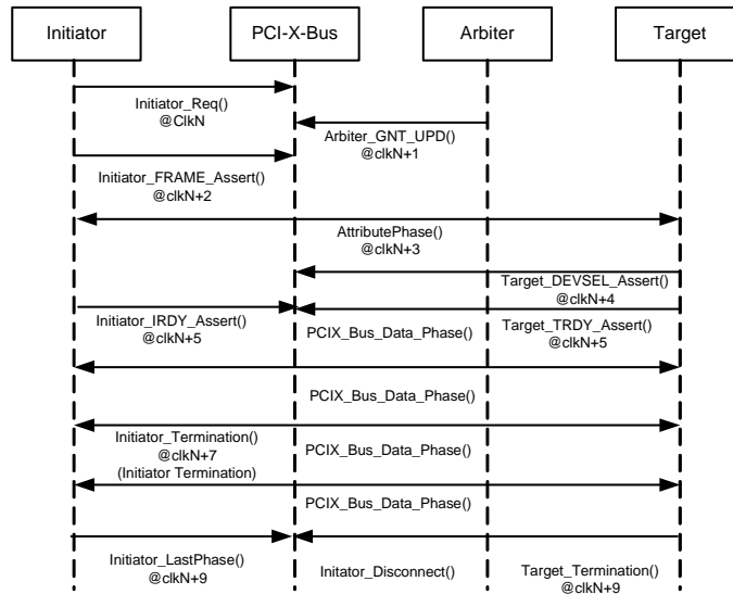
Fig. 7. Sequence Diagram of Mode 1 Transaction.
