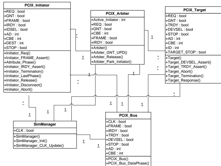
Fig. 6. Class Diagram of PCI-X.
