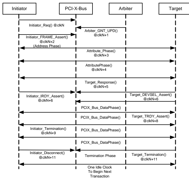
Fig. 9. Sequence Diagram of Mode 2 Transaction (16 bit).
