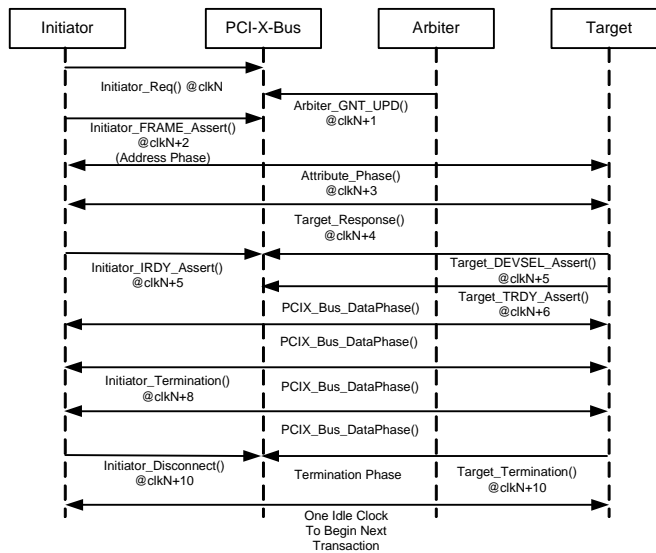
Fig. 8. Sequence Diagram of Mode 2 Transaction.
