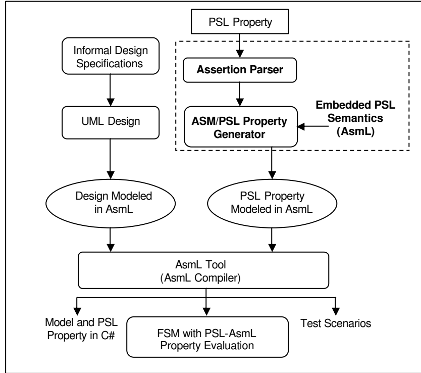
Fig. 1. Design for Verification Methodology based on Embedding PSL in AsmL.
