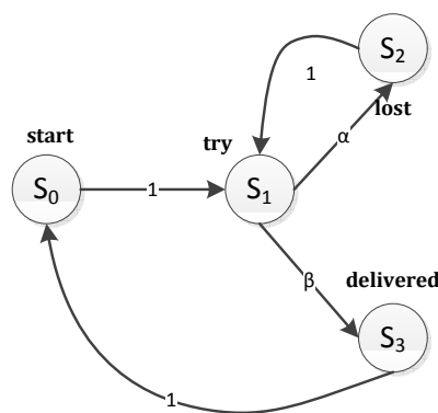
Figure 4: DTMC Model of the AMQM Protocol
