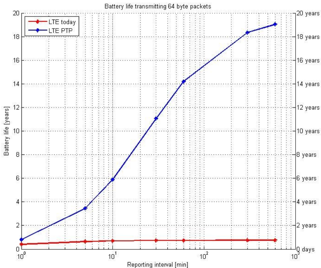
Figure 11: Comparison of baseline battery life
