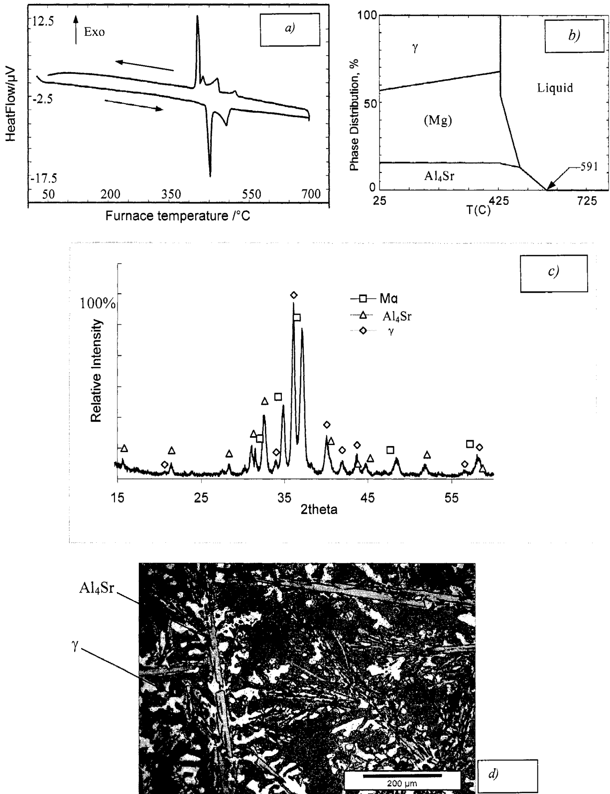
Figure 4-13: a) DSC spectra, b) phase assemblage diagram, c) XRD pattern and d) optical micrograph of sample 4.
