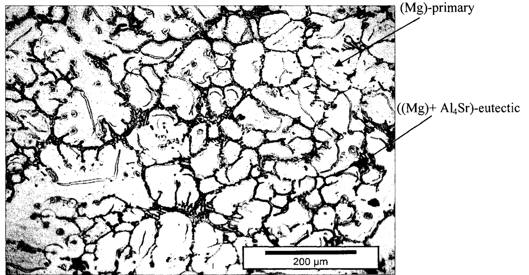
Figure 4-6: Optical micrograph of sample 1.
