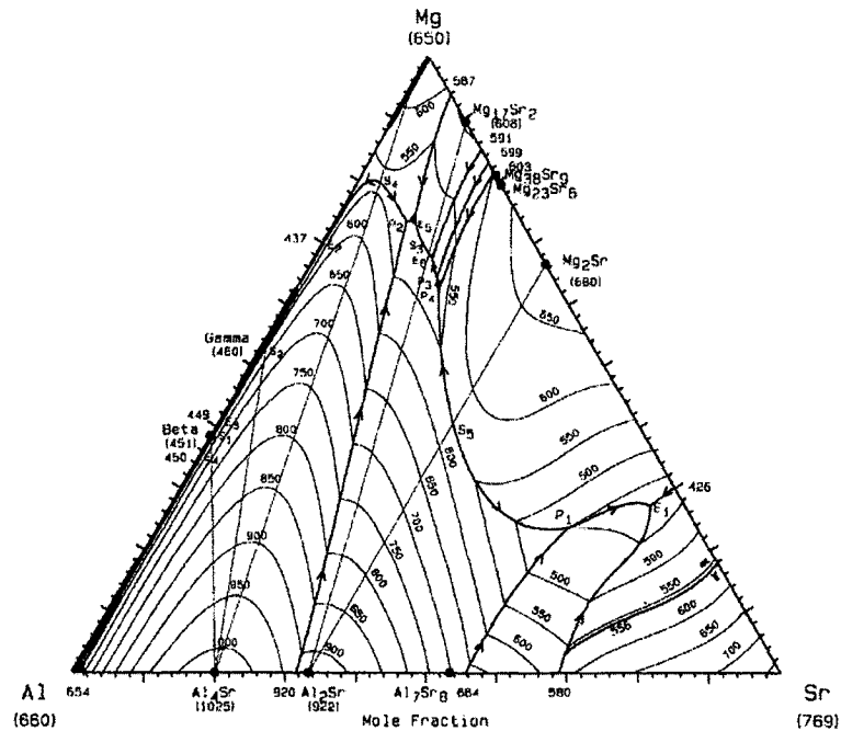
Figure 2-4: Mg-Al-Sr calculated phase diagram in atomic percent [23].
