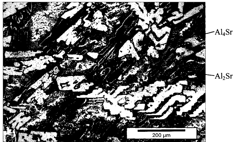
Figure 4-32: Optical micrograph of sample 11.
