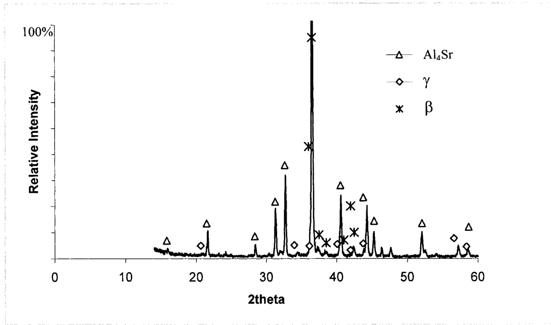
Figure 4-44: XRD pattern of sample 15 (9.5/40/50.5 Sr/Mg/Al wt.%).
