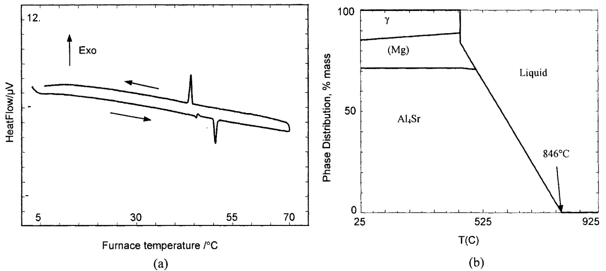
Figure 4-22: (a) DSC spectra and (b) phase assemblage diagram of sample 9.
