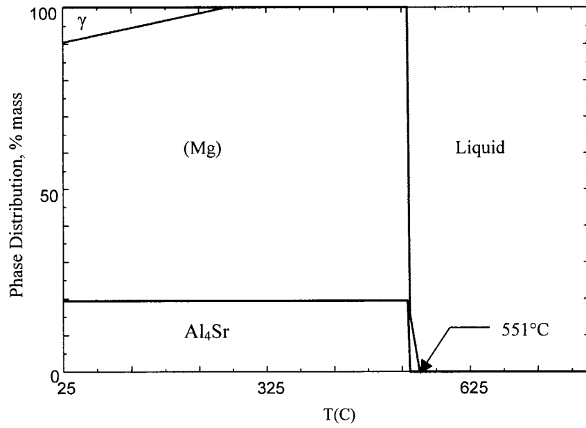
Figure 4-10: Phase assemblage diagram of sample 2.
