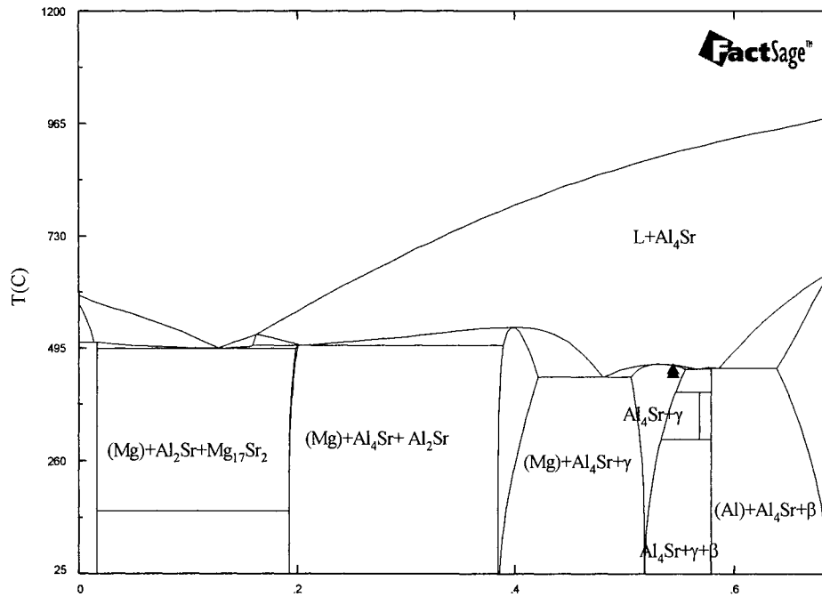
Figure 4-43: Calculated vertical section at constant 31.18 wt.% Sr with DSC signals from cooling curve of sample 17.
