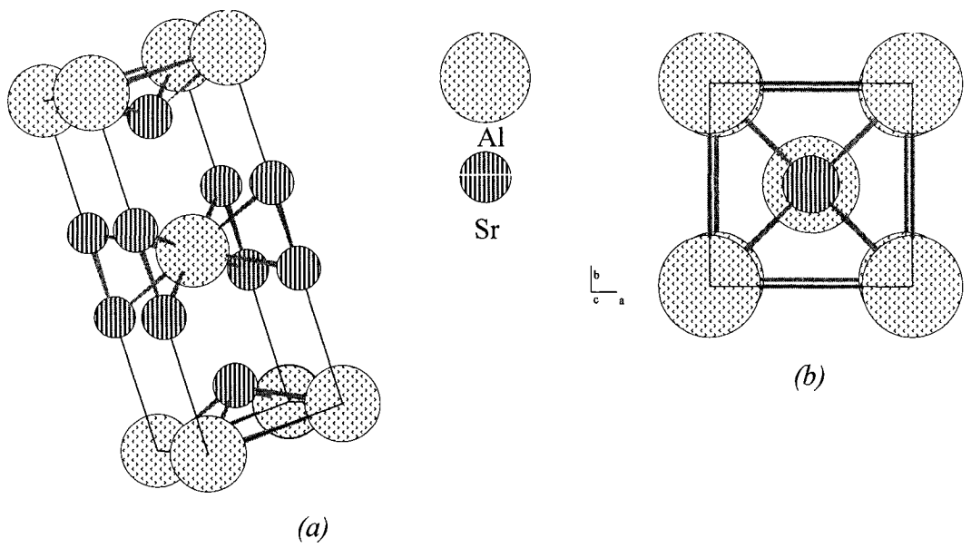
Figure 3-6: (a) Al_4Sr unit cell, (b) (001) projection.
