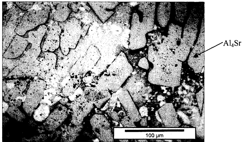
Figure 4-49: Optical micrograph of sample 17.
