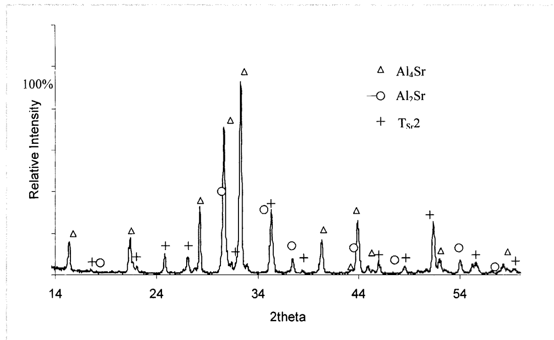
Figure 4-26: X-ray diffraction pattern of sample 11 (27.83/42.89/29.28 Sr/Mg/Al wt.%).
