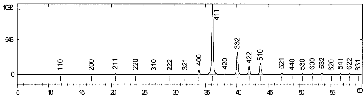
Figure A-4: Calculated XRD diffraction pattern for \gamma .
