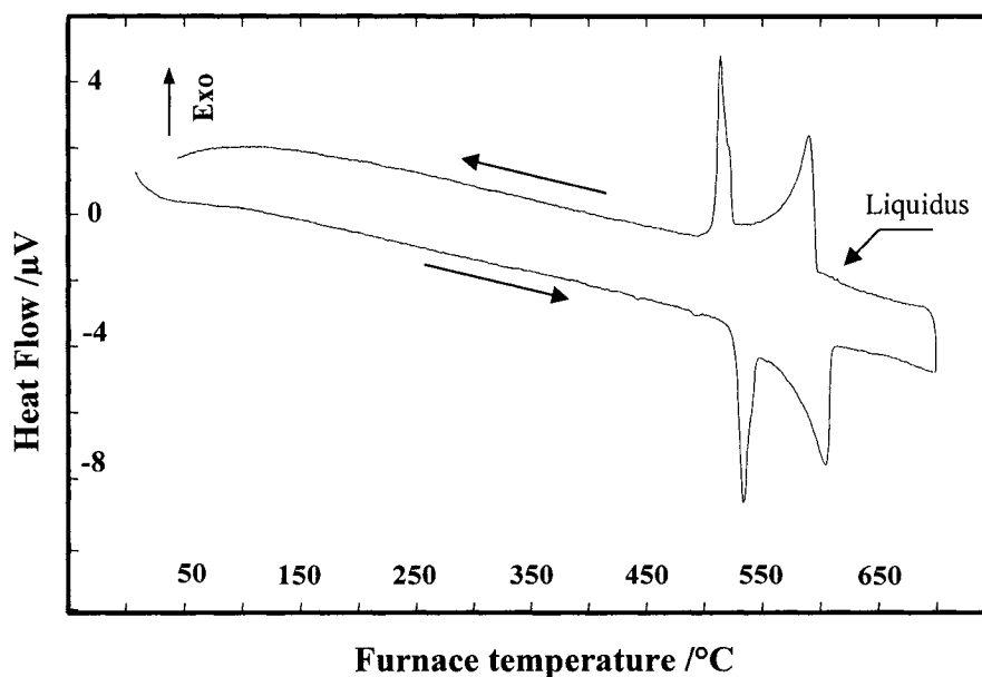
Figure 4-2: DSC spectra of sample 1 (3.32/87.29/9.39 Sr/Mg/Al wt.%) during heating and cooling.
