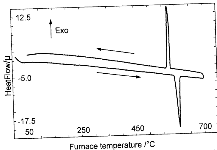
Figure 4-63: DSC spectra of sample 22 (32.74/60.55/6.71 Sr/Mg/Al wt.%) during heating and cooling.
