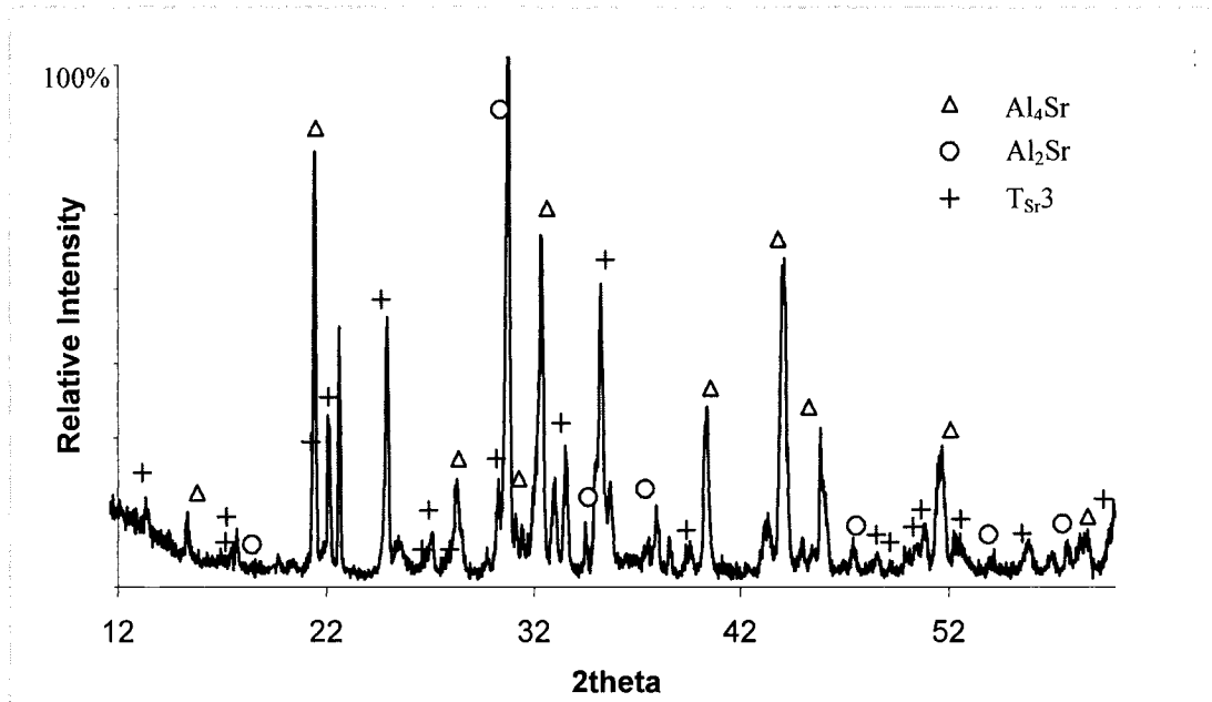
Figure 4-35: X-ray diffraction pattern of sample 13 (39.87/30.73/29.4 Sr/Mg/Al wt.%).
