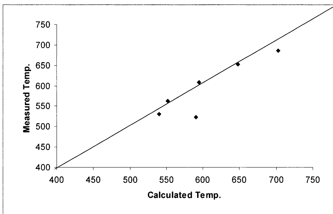
Figure 4-16: Comparison between calculated and experimental DSC data.
