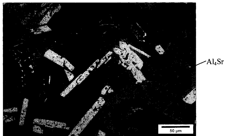
Figure 4-47: Optical micrograph of sample 15.
