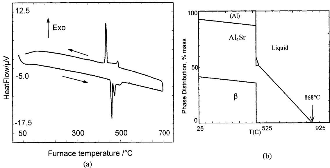
Figure 4-54: (a) DSC spectra and (b) phase assemblage diagram of sample 20.
