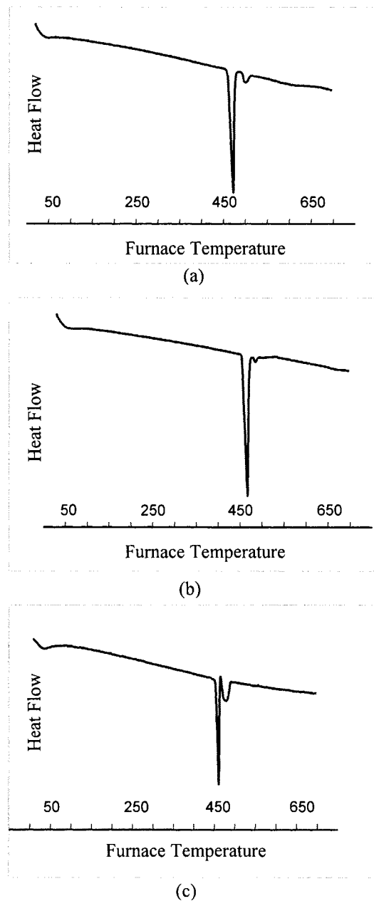
Figure 4-40: DSC traces of the three samples (a) 15, (b) 16 and (c) 17.
