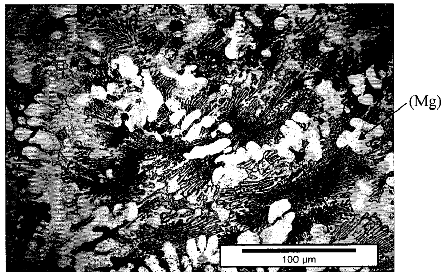
Figure 4-11: Optical micrograph of sample 2.
