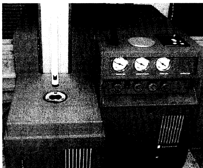
Figure 3-3: Setaram DSC.
