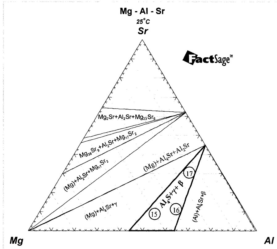
Figure 4-39: Isothermal section at 25°C showing samples in Al_4Sr+\gamma+\beta phase field.
