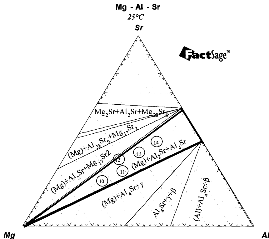
Figure 4-24: Isothermal section at 25°C showing samples in (Mg)+Al 4 Sr+Al 2 Sr phase field.
