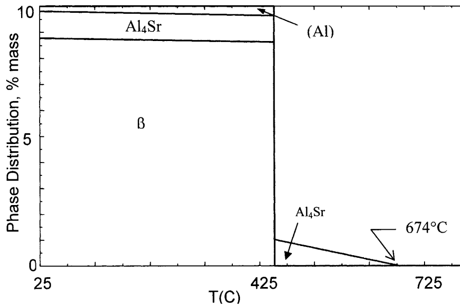
Figure 4-52: Phase assemblage diagram of sample 18.
