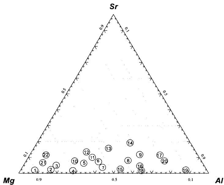
Figure 3-2: Ternary diagram showing investigated compositions in at.%.
