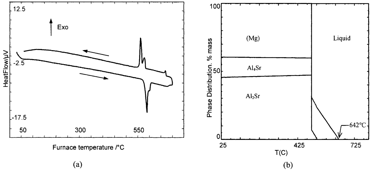
Figure 4-36: a) DSC spectra, b) phase assemblage diagram of sample 12.
