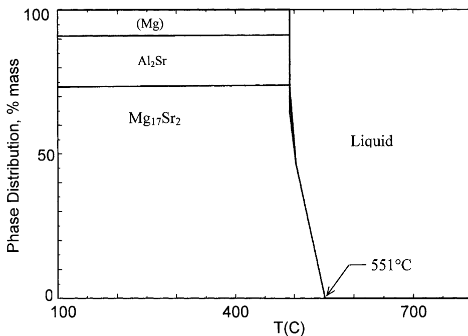
Figure 4-64: Phase assemblage diagram of sample 22.
