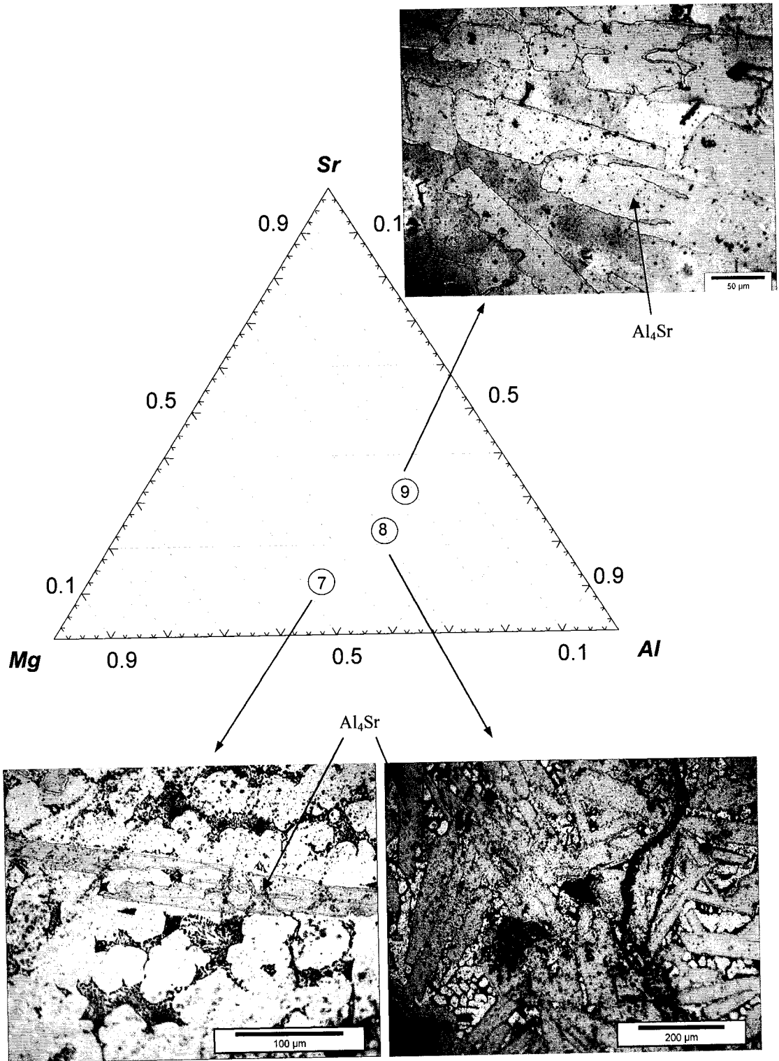
Figure 4-23: Optical microscopic images.
