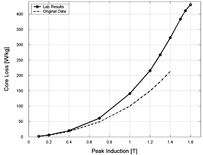
Fig. 13. M45 core losses at 1.0 kHz.
