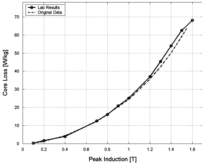
Fig. 11. M19 core losses at 400 Hz.
