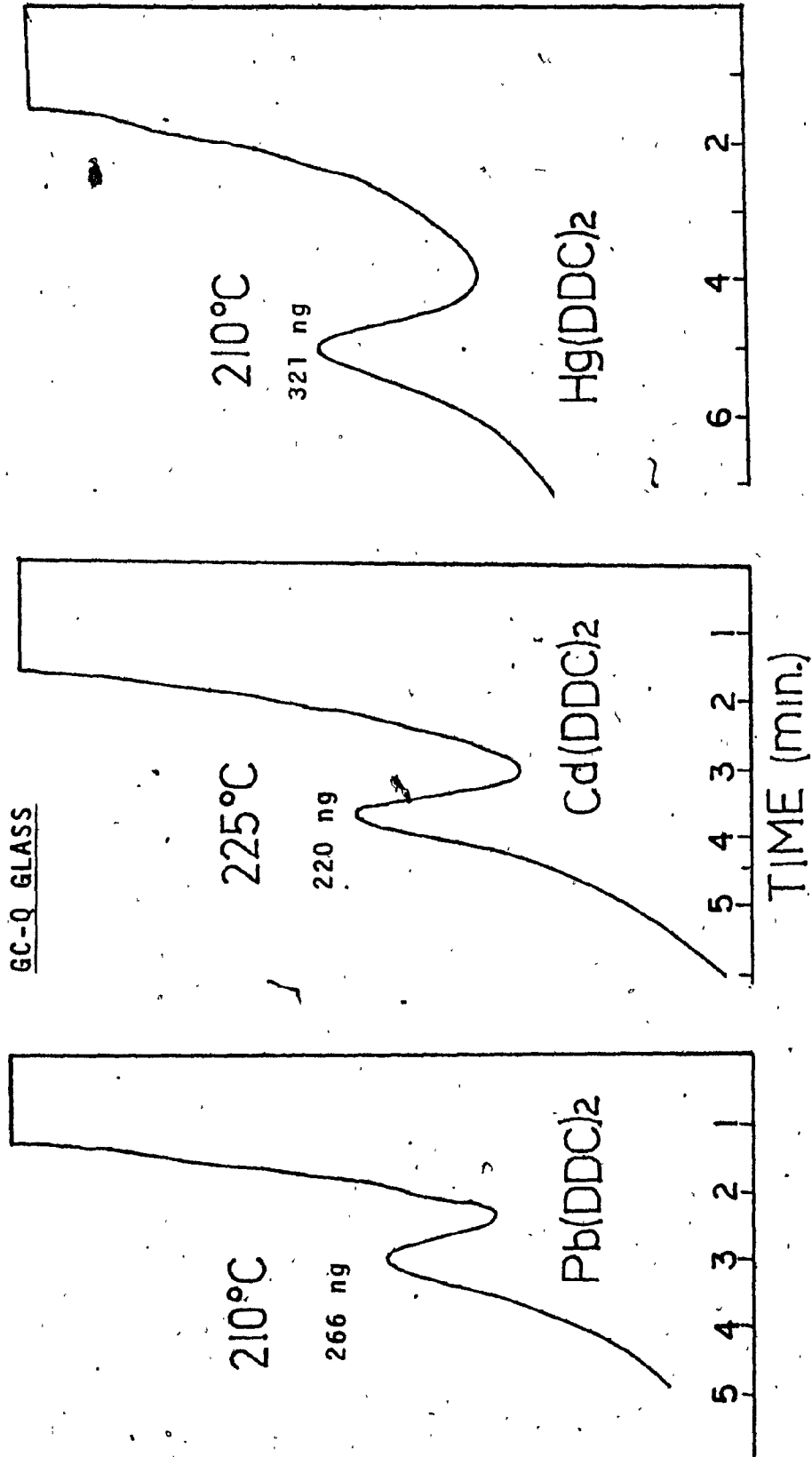
FIGURE 40 PEAK SHAPE OF Pb, Cd and Hg on 2% SE-30 + 2% QF-1 (60 cm x 2 mm) ON GC-Q GLASS
