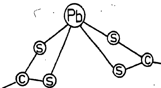
Fig. 7: Pb(DDC)_2 Structure
