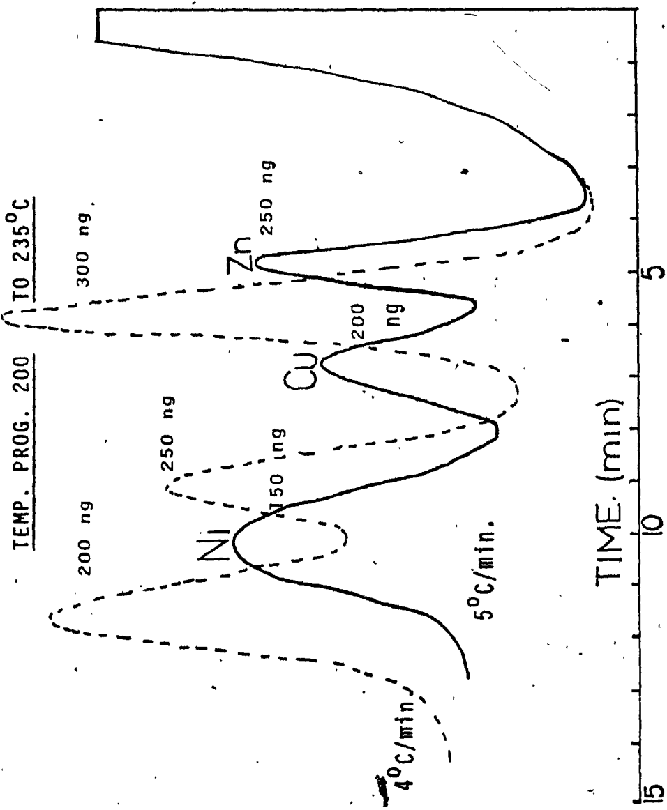
FIGURE 37 SEPARATION OF H(DDC)_2 ON 2% SE + 2% OV-17 ON CM-HP (40 cm x 1/8")
