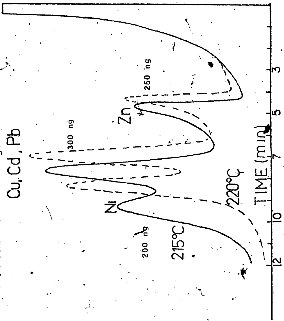
FIGURE 21(B) SEPARATION ON 5% OV-101 ON CM-AW-DMCS (50 \mu m x 1/8" S.S.)
