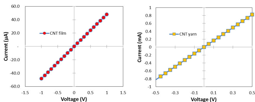
Fig. 5. Current-voltage (IV) characteristics of the pressure sensors. (a) Carbon nanotube web/film. (b) Carbon nanotube yarn.
