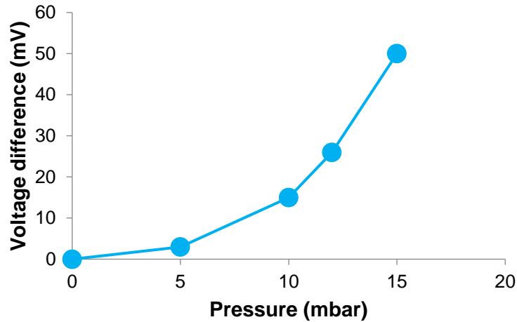
Fig. 8. Pressure sensing characteristics of the CNT film pressure sensors
