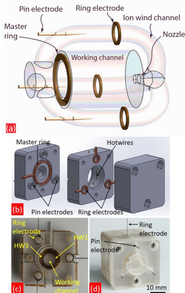
Figure 1. Present point-to-ring corona based gyroscope: (a) Schematic design, (b) 3D sketch and (c, d) experimental prototype.
