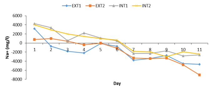
Figure 9b Changes of sodium ion ( \text{Na}^+ ) in the green roof effluents ( \text{Na}^+ of raw greywater – \text{Na}^+ of effluent).
