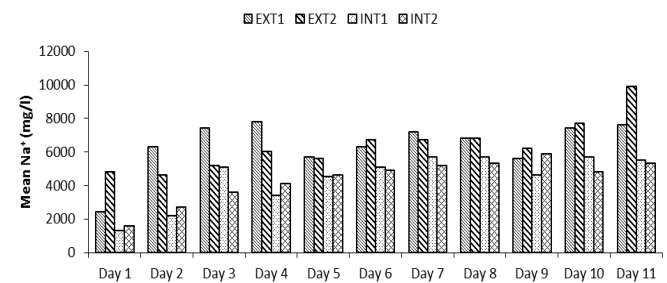
Figure 9a Mean sodium ions ( \text{Na}^+ ) of green roof effluents.
