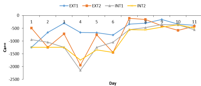
Figure 8b Changes of calcium ions ( \text{Ca}^{++} ) in the green roof effluents ( \text{Ca}^{++} of raw greywater – \text{Ca}^{++} of effluent).
