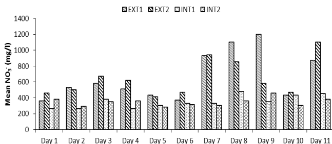
Figure 11a Mean nitrate (as NO_3^- ) of green roof effluents.
