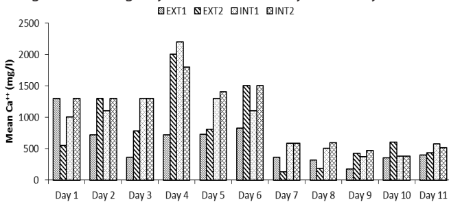
Figure 8a Mean calcium ion ( \text{Ca}^{++} ) concentration of green roof effluents.
