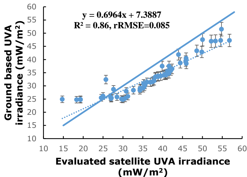
Figure 5. Comparison of the broadband UVA irradiances evaluated from OMI spectral data and the UVA irradiance from the ground based measurements were derived from Equation 2 to use the OMI spectral irradiances. The error bars are the \pm 10\% error associated with the ground based data and the solid line is the 1:1 line.
