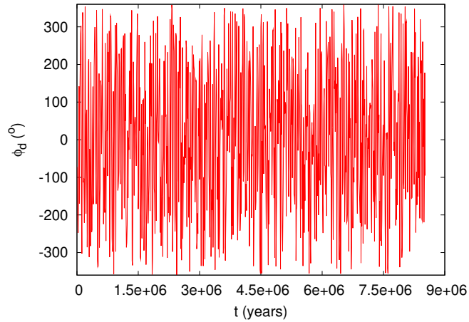
Fig. 4: Variation in the resonant argument \phi_d given by Eq. 4 for the longest living test particle at 1.5 AU of model 4.
