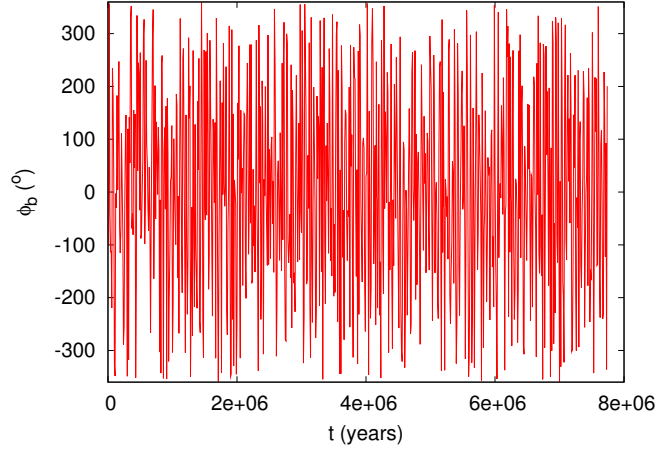
Fig. 3: Variation in the resonant argument \phi_b given by Eq. 3 for the longest living test particle at 1.4 AU of model 4.
