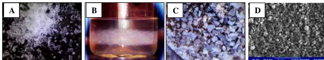
Figure. 2 (A) The hydrogel, (B) two phases formed at the end of surface modification step, (C) the aerogel granules, and (D) SEM micrographs
