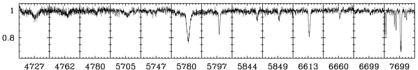
Figure 7. Preliminary data on DIBs and on the K I interstellar atomic line at 7699\text{ \AA} as observed by GALAH. Spectrum of TYC 4011-102-1, a hot star with strong interstellar absorptions close to the Galactic plane, is shown. Each 20\text{ \AA} wide panel is centred on the DIB wavelength as listed in Jenniskens & Desert (1994). Plotted wavelengths are heliocentric. Right-most panel identifies two interstellar clouds for K I at different velocities. For a majority of GALAH objects which lie away from the Galactic plane such complications are rare (but can be detected).
