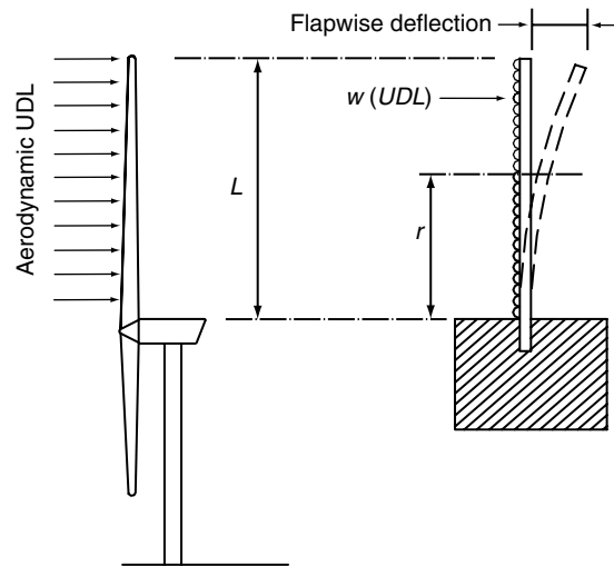
Figure 10: The blade modelled as a cantilever beam with uniformly distributed aerodynamic load.
