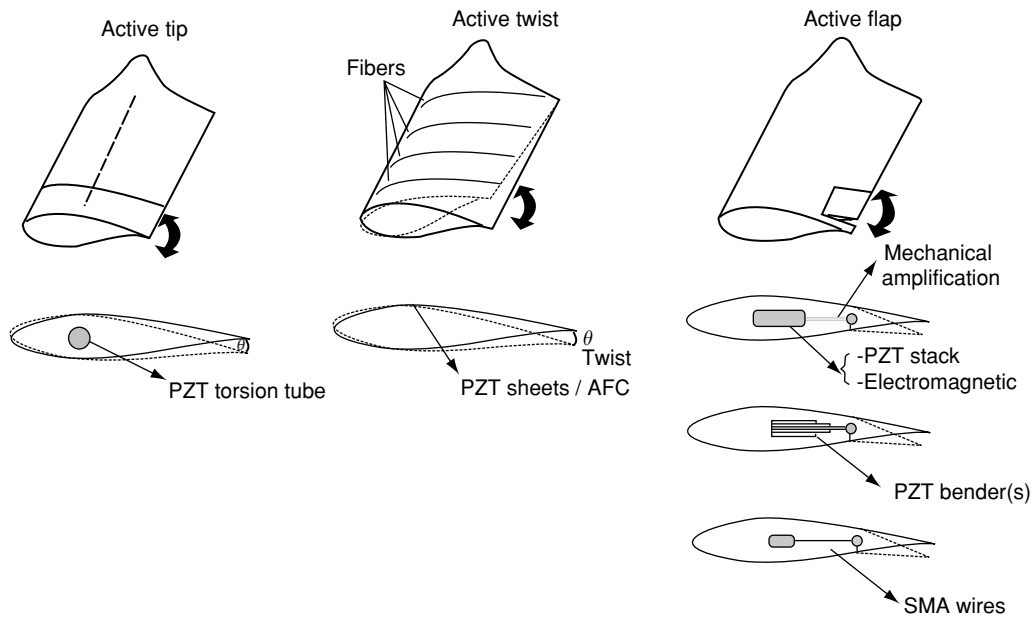
Figure 6: Schematics of smart structure concepts.
