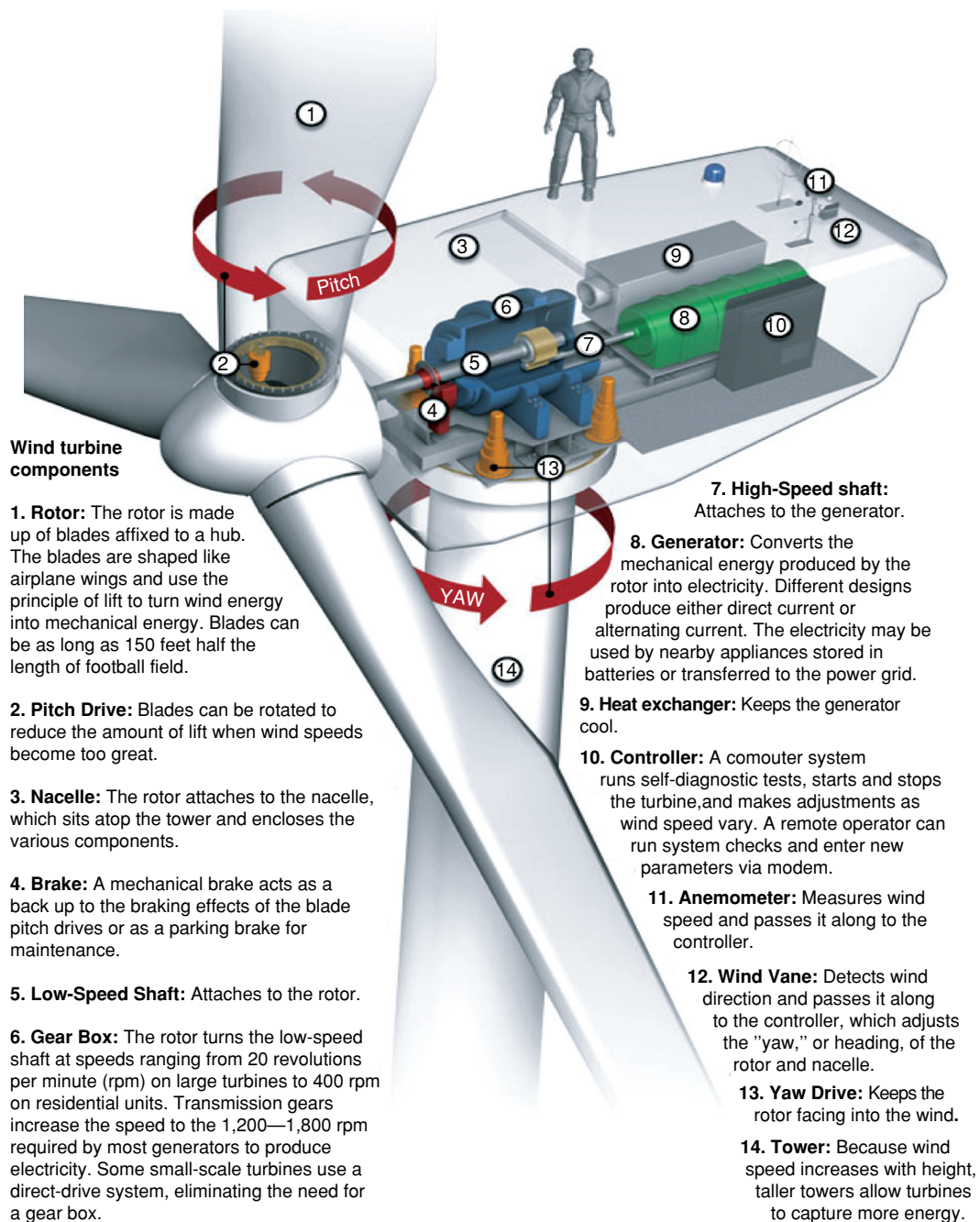
Figure 5: Typical configuration of a modern large scale wind turbine [www.desmoinesregister.com].
