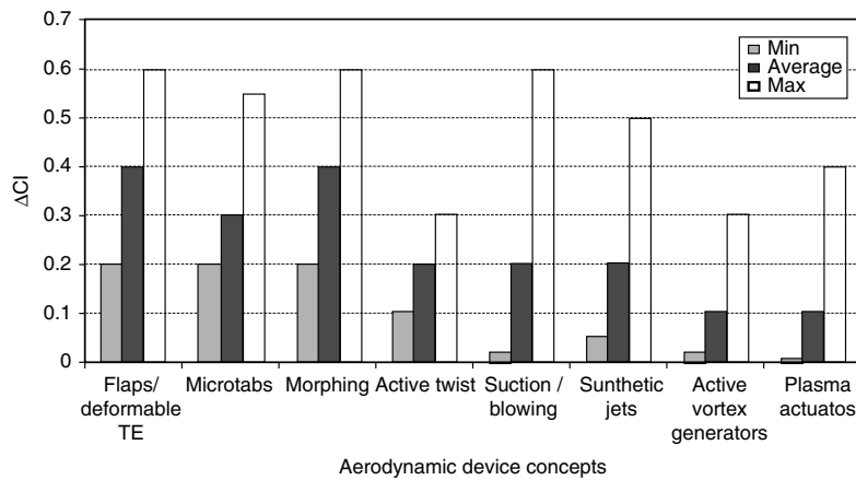
Figure 7: Comparison of aerodynamic device concepts in terms of lift control capability [31].
