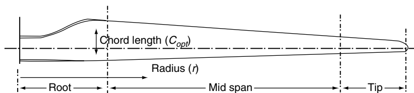
Figure 2. A typical blade plan and region classification.
