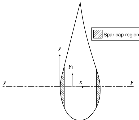
Figure 13: Edgewise bending about yy .
