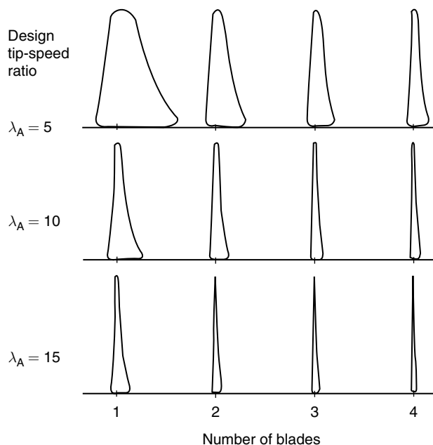
Figure 3: Optimal blade plan shape for alternate design tip speed ratios and number of blades [1].
