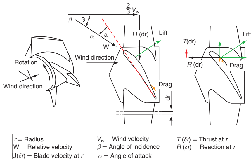
Figure 9: Aerodynamic forces generated at a blade element.
