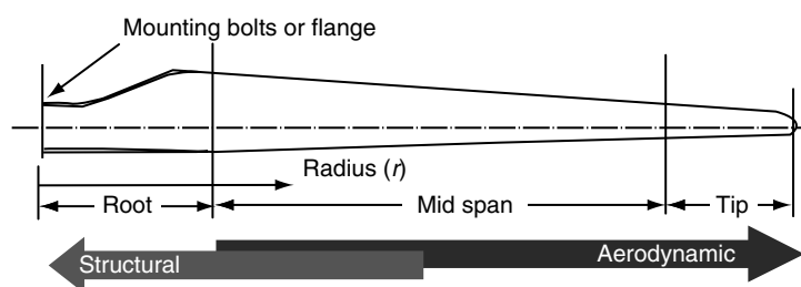
Figure 14: The three blade regions.
