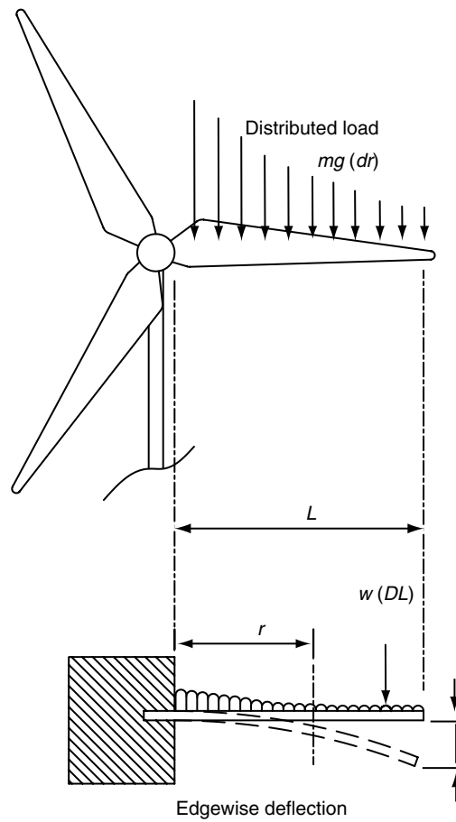
Figure 12: Gravitational load modelled as a cantilever beam.
