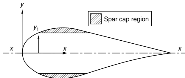
Figure 11: Flapwise bending about the axis xx.
