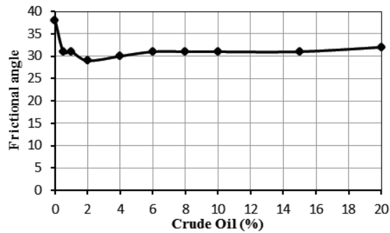
Figure 5: Frictional angle as a function of the percentage of crude oil contamination (%)
