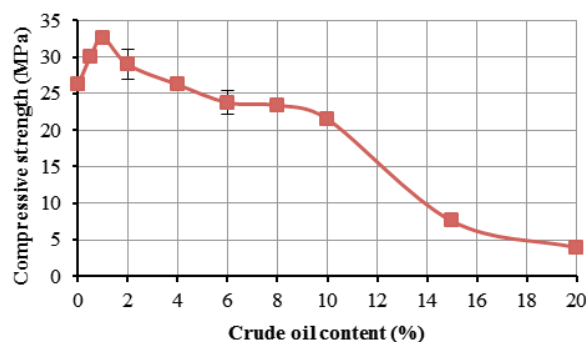
Figure 6: Effect of different crude oil content on the compressive strength
