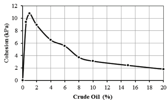
Figure 1: Cohesion as a function of crude oil contamination percentage (%)
