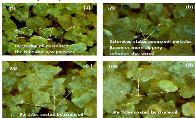
Figure 3: Images of fine sand with different percentages of contamination (4 to 10%)
